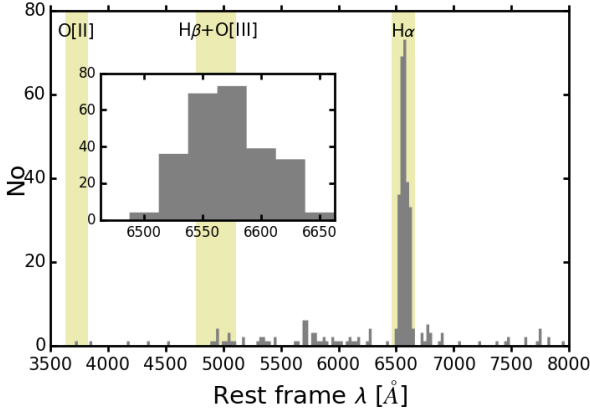
Figure 5. Histogram of the distribution of emitters with spectroscopic redshift. Because of the different NB filters tracing different redshift ranges, we transform into the rest-frame of the main emission line. The ranges for which H\alpha , O[II] , H\beta and O[III] emitters are expected to be picked up by our filters are marked with the shaded areas. The distribution is clearly dominated by H\alpha emitters indicating the filters properly select emitters. Note however, that most of the spectra were targeting the red sequence of the clusters, hence the number of emitters with spectra is rather low. However, the chance of an emitter at the cluster redshift to have a spectrum is still much larger than if they were at a higher redshift, hence there is a bias in source redshifts. The number of spectra for sources at different redshift from the cluster distance is therefore lower than in reality.
