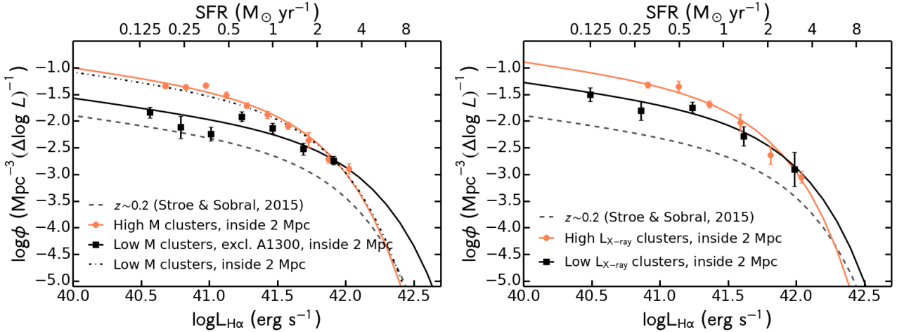
Figure 10. The H \alpha LF for stacks of low and high mass cluster (left panel) and low and high luminosity clusters, respectively (right panel). Only the emitters within 2 Mpc of the cluster centre were considered. There is marginal evidence for X-ray bright clusters hosting more numerous, lower luminosity H \alpha emitters on average. There are no differences between the low and high mass cluster LF, when A1300 is included in the low-M ‘stack’.
