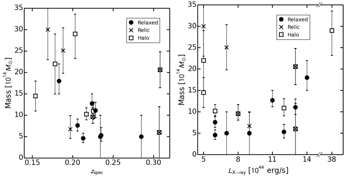
Figure 1. Distribution of galaxy clusters with respect to mass and redshift (left panel) and with respect to mass and X-ray luminosity (right panel). The relaxation state is encoded in the symbol. Note that masses are inferred from weak lensing estimates when available, but in some cases such an estimate was not available so we use the total mass estimate based on the cluster’s velocity dispersion. Note the lack of correlation between mass and luminosity, especially for the disturbed clusters.
