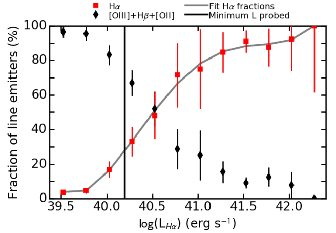
Figure 6. Fraction of H\alpha emitters expected from a population of line emitters selected with a NB survey, as function of H\alpha luminosity. The gray line displays the H\alpha fraction fit as a function of the luminosity.
