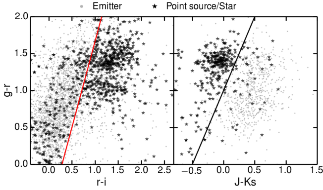
Figure 4. Colour-colour plots for emitters. The left plot displays the g-r colour versus r-i . The right plot represents g-r versus J-Ks . Point-like objects are represented with stars, while emitters are shown in gray dots. The lines show the colour cuts used to select point-like objects, in combination with other criteria as discussed in Section 4.2.
