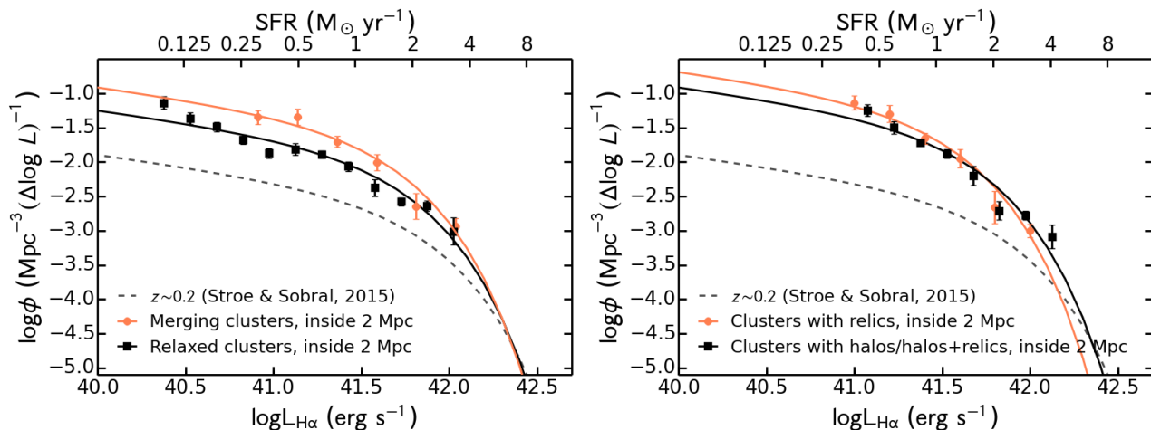
Figure 9. Left panel: The H\alpha LF for merging and relaxed clusters (within 2 Mpc of centre). Note the differences in normalisation of the two LFs. Right panel: The H\alpha LF for clusters hosting relics and haloes, respectively (within 2 Mpc of centre). The presence of shocks mildly boosts the number of H\alpha emitters compared to a cluster hosting a halo.
