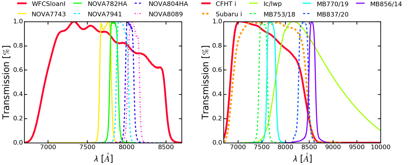
Figure 2. Normalised profiles of the NB filters used to survey H\alpha emitters at the redshift of our clusters. The BB filters used for continuum subtraction are also overplotted.
