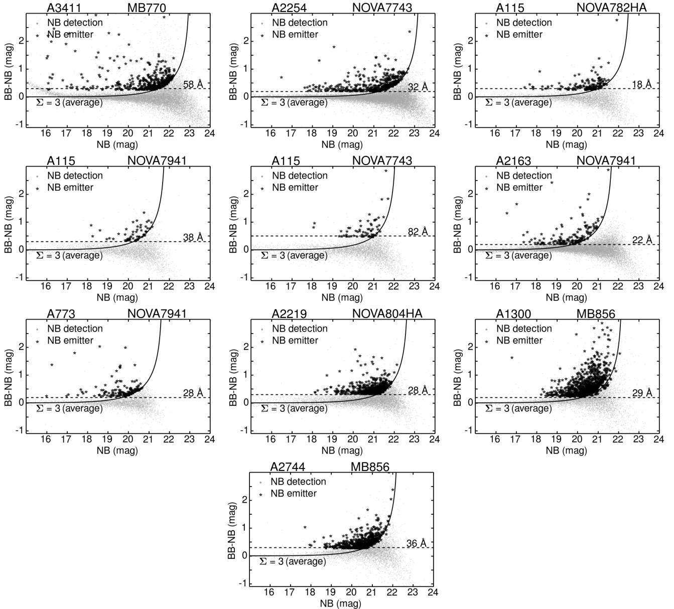
Figure 3. (cont.) Colour-magnitude diagrams of the colour excess as function of NB magnitude. We select emitters separately on each CCD for each cluster and adapt the cuts to reflect the noise levels reached in each observation. The curve represent the average 3\Sigma colour significances and the dashed, black line represents the restframe EW_0 cut.
