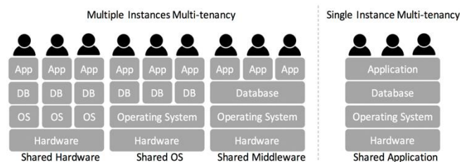
Figure 1. Multi-tenancy patterns
