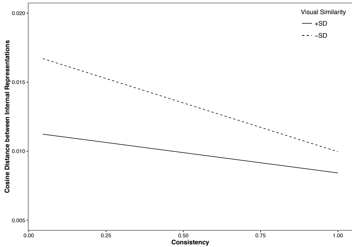
Figure 8. Cosine distance between internal representations for all phonetic radical families as a function of consistency and visual similarity.
