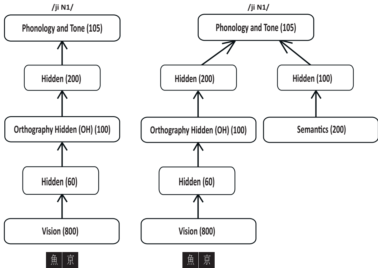
Figure 1. The architectures of the VP model (left panel) and the VSP model (right panel).
