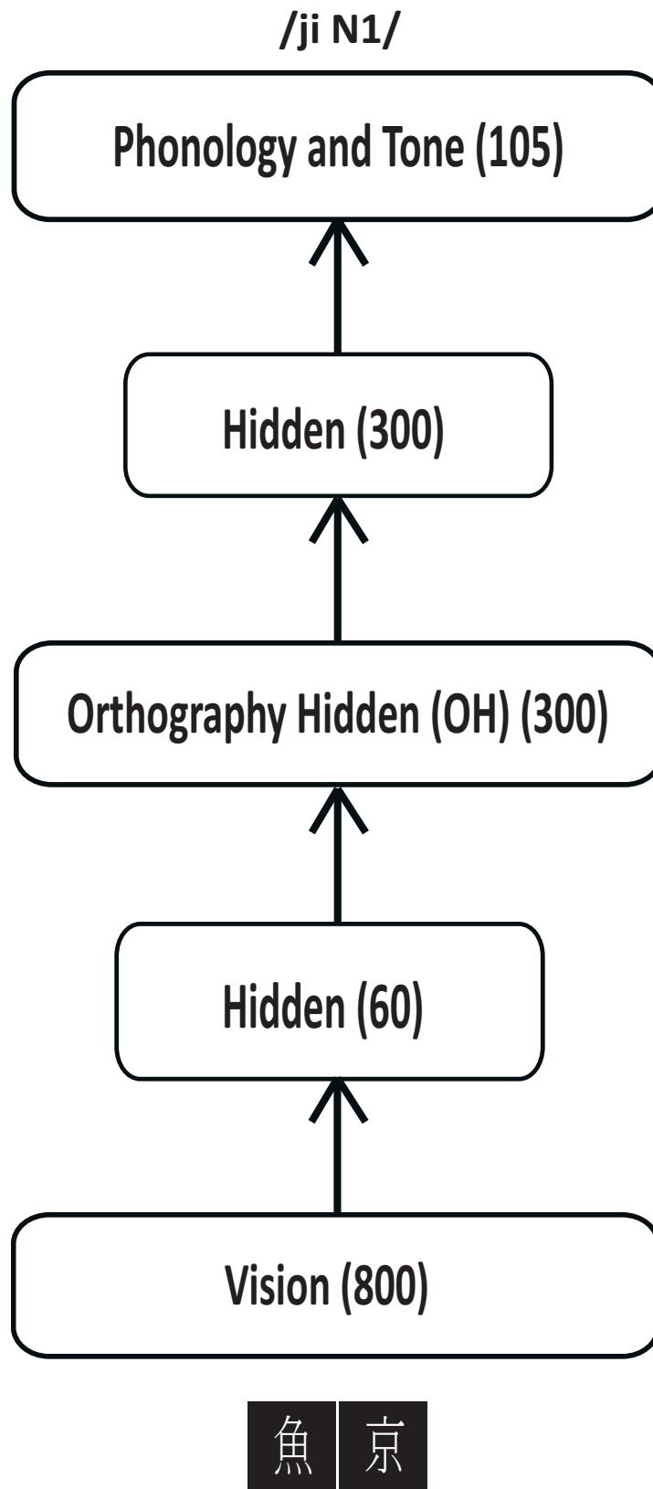
Figure A1. The architecture of the VP control model.
