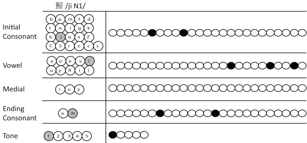
Figure 2. The phonological representation scheme based on Chinese phonetic features.
