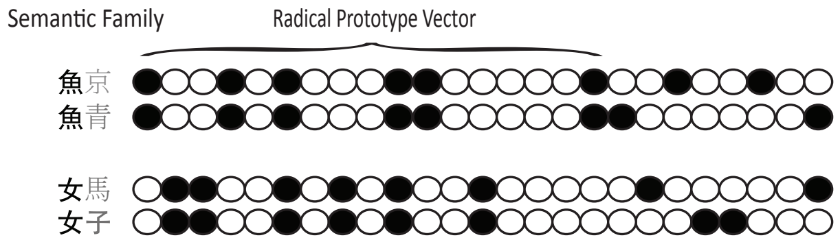
Figure 3. Illustrations of semantic representations used in the VSP model.
