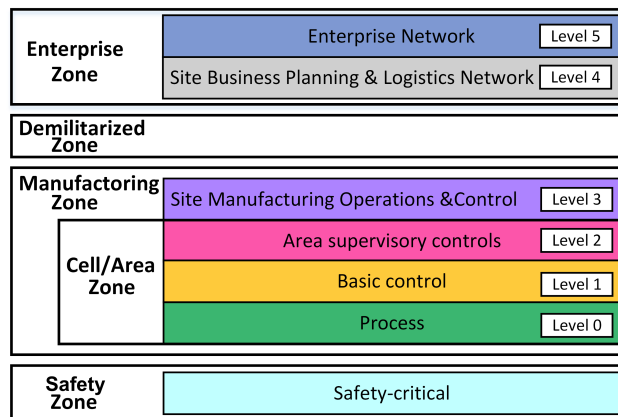
Figure 1: The Purdue Model [16]
