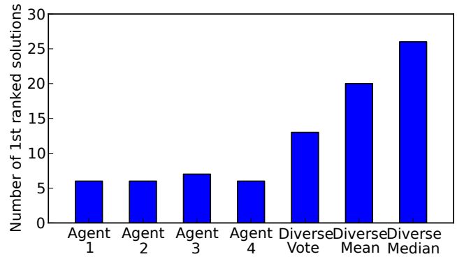
Figure 4: Number of 1st ranked solutions, for each agent and the diverse team.
