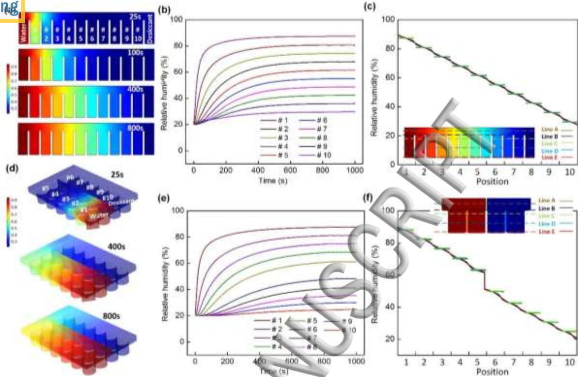
FIG 2. Simulated dynamic process to generate discrete humidity gradients in the I-shaped and U-shaped devices. (a) and (d) give time-lapse images of water vapor movement inside the devices at different time points. (b) and (e) plot simulated relative humidity as a function of time in each well of the I-shaped (b) and U-shaped (e) devices. The wells of the I-shaped and U-shaped devices are numbered from #1 to #10 as shown in (a) and (c), respectively. The water and drying agent reservoirs are not numbered. (c) and (f) give simulated steady-state relative humidity gradient in the continuous top layer (line A), at the interface (line B) between the top and bottom layer, and at the three different depths (lines C-E) in the well bottom layer, of the I-shaped (c) and U-shaped (f) devices, respectively.
