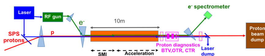
Fig. 2. Baseline design of the AWAKE experiment.
