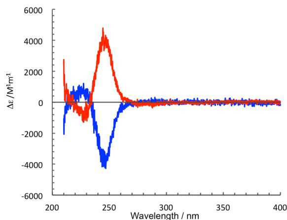
Fig. 6 Circular Dichroism spectra of (a) S -1 (blue) and (b) R -1 (red) obtained following extraction from the salts of 1- D -DTT and 1- L -DBT respectively (8x10 -5 mol dm -3 in methanol 293 K).
