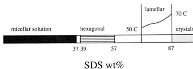
Figure 1.10 Surfactant-water phase diagram for SDS at 40°C. Blank areas correspond to two phase regions. The lamellar phase at higher than 50°C is also show. Reprinted with permission from Marques 1993. Copyright 1993 American Chemical Society. 99
