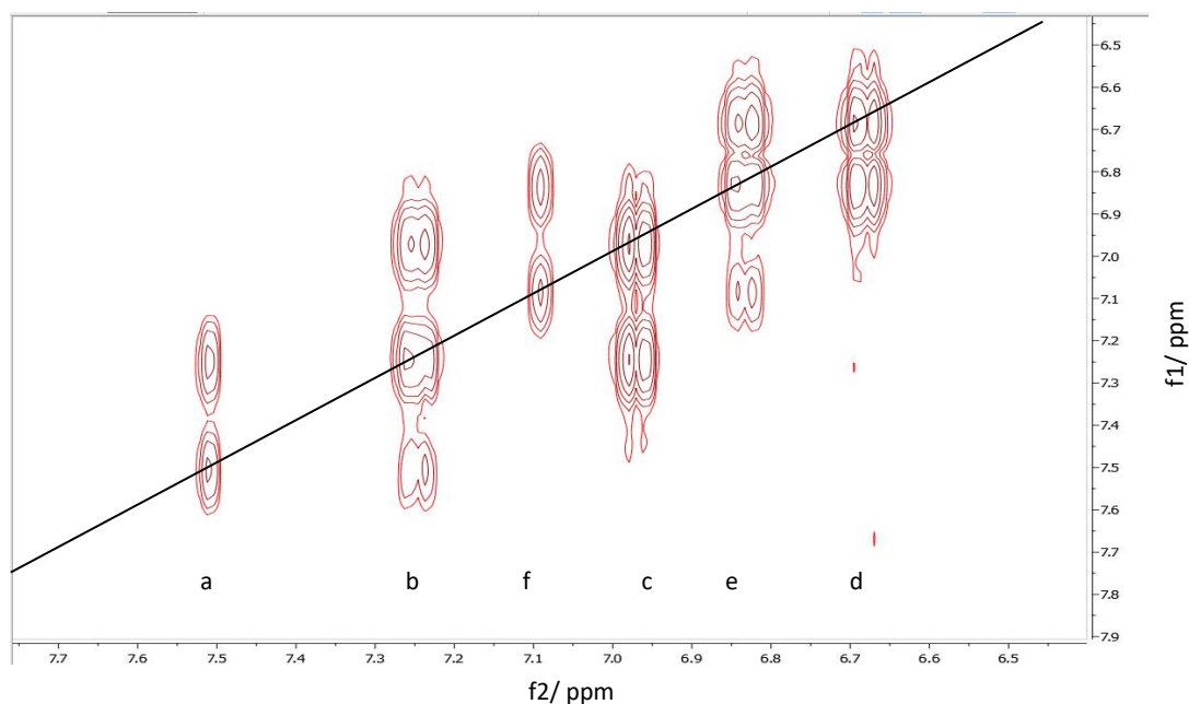
Figure 3.5 400 MHz ^1\text{H} COSY spectra of TC in \text{CDCl}_3 : \delta 7.4743 (d, J = 2.5 Hz, 1H, a), 7.2120 (dd, J = 8.8, 2.6 Hz, 1H, b), 7.0565 (d, J = 2.5 Hz, 1H, f), 6.9339 (d, J = 8.8 Hz, 1H, c), 6.7985 (dd, J = 8.7, 2.5 Hz, 1H, e), 6.6464 (d, J = 8.7 Hz, 1H, d).
