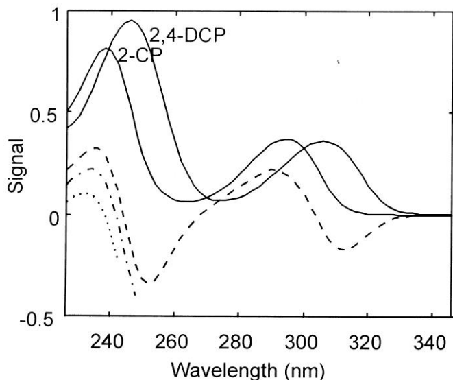
Figure 8.4 Absorbance spectra of 2,4- DCP and 2-chlorophenol (2-CP) in water. Reprinted with permission from Ferré 1998. Copyright 1998 American Chemical Society. 238
