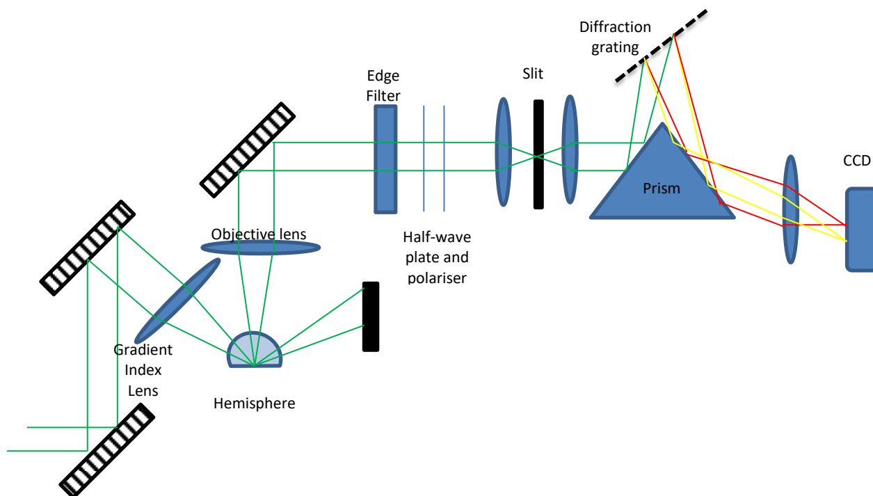
Figure 4.8 The collection optics of the Renishaw TIR-Raman Spectrometer
