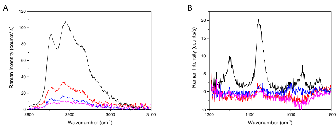
Figure 4.60 TIR-Raman spectra collected at 2900\text{ cm}^{-1} (A) and 1600\text{ cm}^{-1} (B) using S polarised light of a 1.2:1 POPC/ POPG bilayer (black) in pH 7.4 Tris buffer with 2\text{ mM CaCl}_2 . The bilayer was treated with 0.12\text{ mg/mL} TC at pH 10.8 for half an hour (red) and rinsed with 20\text{ mL} of pH 7.4 buffer with 2\text{ mM CaCl}_2 (blue) and an extra 100\text{ mL} of buffer (pink). Laser power was 300\text{ mW} .
