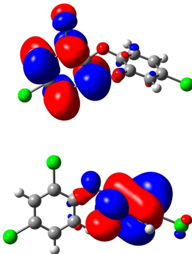
Figure 2.5 Electron density plots of the LUMO (above) and the HOMO (below) orbitals of TC. Reprinted with permission from Kliegman 2013. Copyright 2013 American Chemical Society. 216
