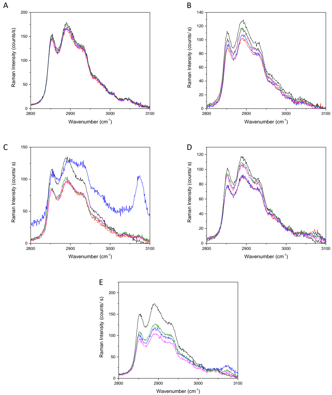
Figure 4.23 TIR-Raman spectra collected at 2900\text{ cm}^{-1} using S polarised light of a POPC bilayer (black) in pH 7.4 Tris buffer with 2\text{ mM CaCl}_2 . The bilayer was treated with different concentrations of TC in pH 10.8 buffer and left for 15 minutes (red). The bilayer was rinsed with 20\text{ mL} of pH 7.4 Tris buffer with 2\text{ mM CaCl}_2 (blue) and with a further 100\text{ mL} of pH 7.4 buffer (pink) and left for an hour (green). The bilayers was treated with the following concentrations of TC: 0.01\text{ mg/ mL} (A), 0.05\text{ mg/ mL} (B), 0.2\text{ mg/ mL} TC (C), 0.3\text{ mg/ mL} TC (D) and 0.4\text{ mg/ mL} TC (E). Laser power was 300\text{ mW} .
