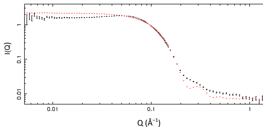
Figure 8.1 Scattering intensity I(Q) in \text{cm}^{-1} of 1.98% SDS, 0.02% TC in 0.1 M NaCl, 0.01 M NaOAc (black) against wave vector transfer, Q in \text{\AA}^{-1} and fitting (red)
