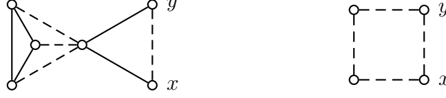
Figure 4.5: Strong negators: the dashed lines represent blue negators in the left graph and red negators in the right. Their endpoints are the vertices x and y from these negators.
