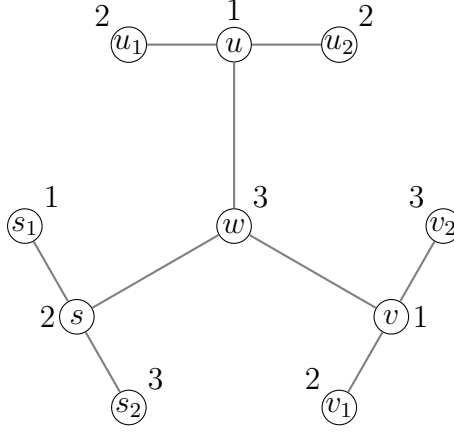
Figure 3.5: The colouring \alpha of Case 3 of Lemma 3.6.
