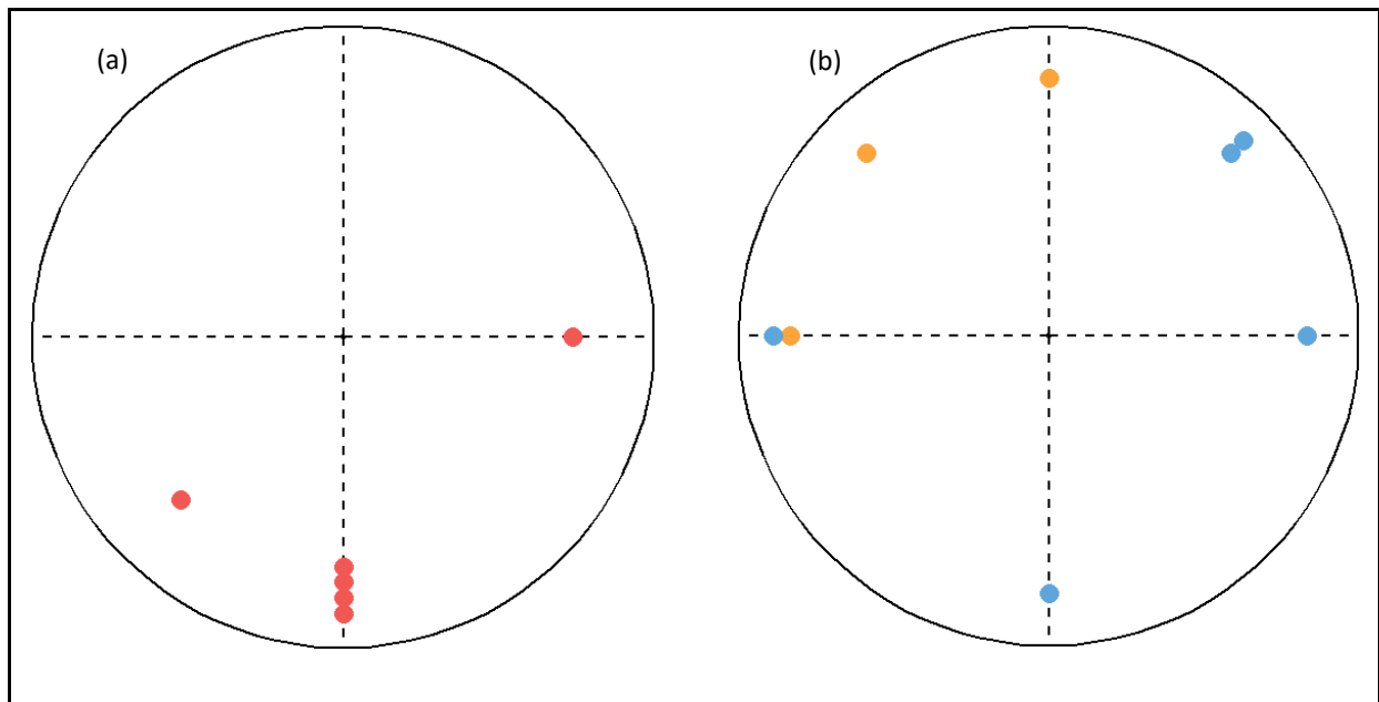
Figure 2. Initial movement directions of leopards following playbacks. This figure shows the initial bearings of movement (relative to speaker locations) of leopards following roar a (red), hornbill b (orange) and dummy b (blue) playbacks. Movement directions were recorded for all moving leopards regardless of the length of time after playbacks that movement began. Instances where leopards did not move, (roar: n = 1, hornbill: n = 3; dummy: n = 1) are not shown on this figure. Figures are centred on the leopard's experimental location, with the speaker location north of the centre. Distance travelled is not represented on this figure.
