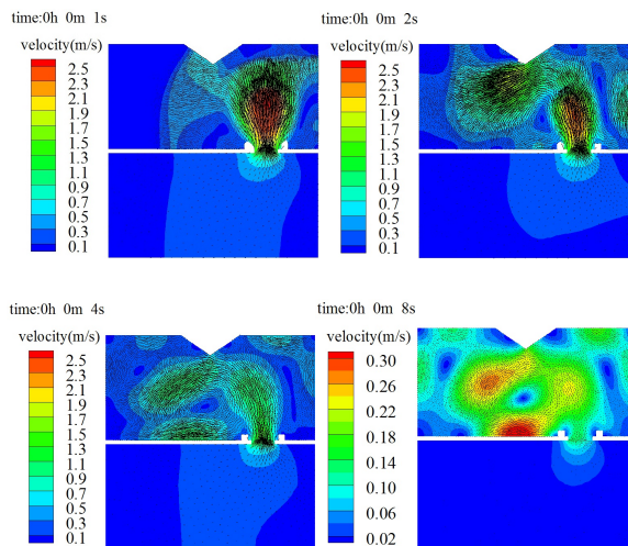
Figure 6. (d) Computed velocity fields of dambreak flow by using fully implicit scheme.
