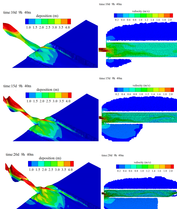
Figure 11. Sediment depositions (left) and flow velocity fields (right) at entrance of plain river.
