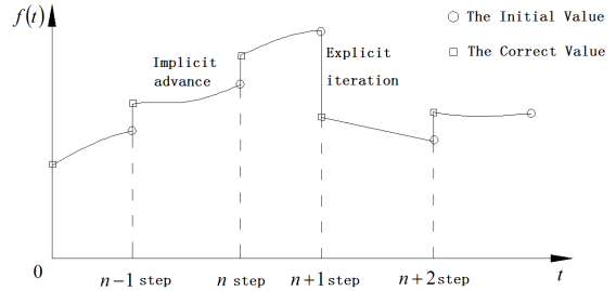
Figure 3. Schematic illustration of coupled explicit-implicit computations.
