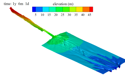
Figure 13. (a) Long-term topographic evolutions of downstream meandering river.
