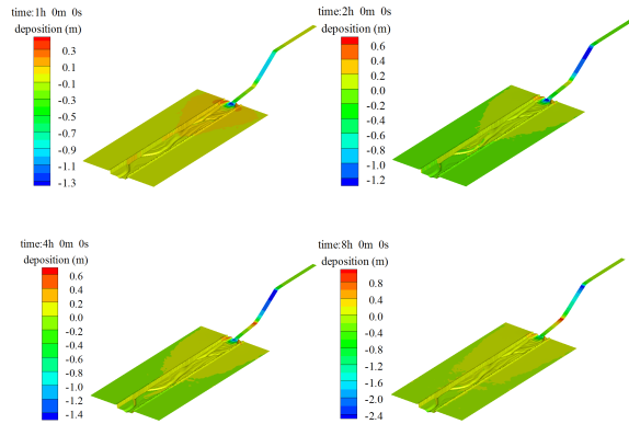
Figure 10. Short-term sediment deposition contours after dambreak.
