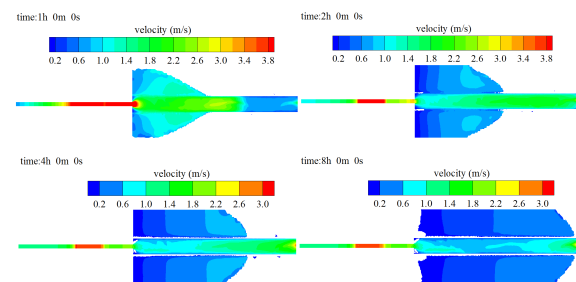
Figure 9. (b) Short-term velocity field contours after dambreak.
