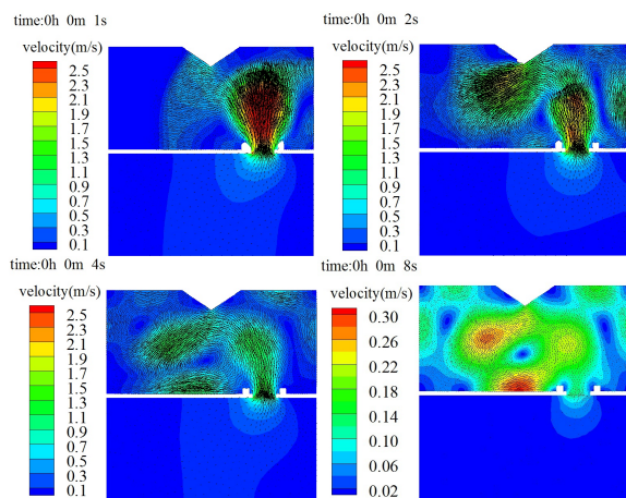
Figure 6. (b) Computed velocity fields of dambreak flow by using coupled explicit-implicit scheme.
