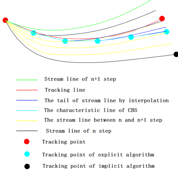
Figure 4. Schematic view of stream/trace lines in a coupled computation.
