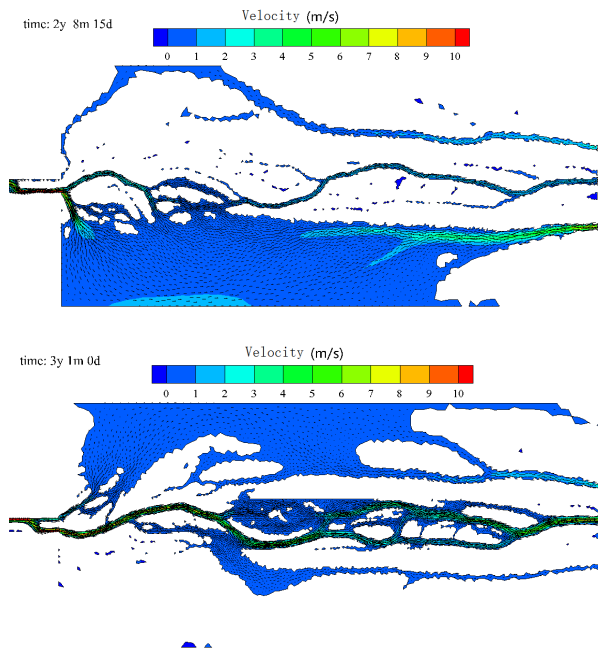
Figure 14. (b) Velocity field of very long-term (3 years) alluvial process and river meandering.
