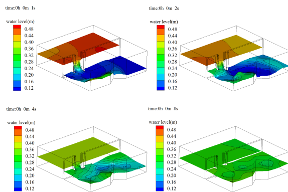
Figure 6. (a) Computed water surfaces of dambreak flow by using coupled explicit-implicit scheme.
