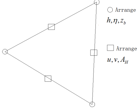
Figure 2. Layout of computational nodes and variables.
