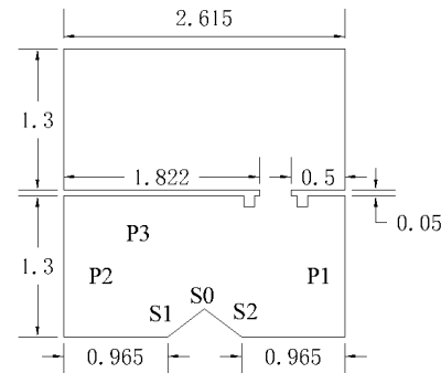
Figure 5. Schematic layout of dambreak flow test (Brufau et al., 2004).
