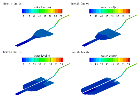
Figure 9. (a) Short-term water level contours after dambreak.
