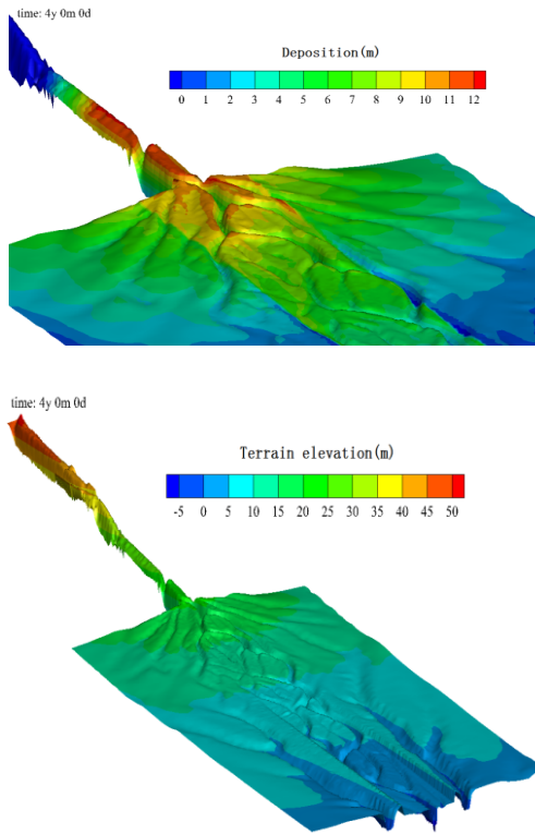
Figure 14. (a) Topography of very long-term (4 years) alluvial process and river meandering.
