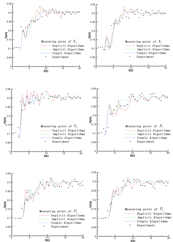
Figure 7. Computed and measured water level variations of dambreak flow
