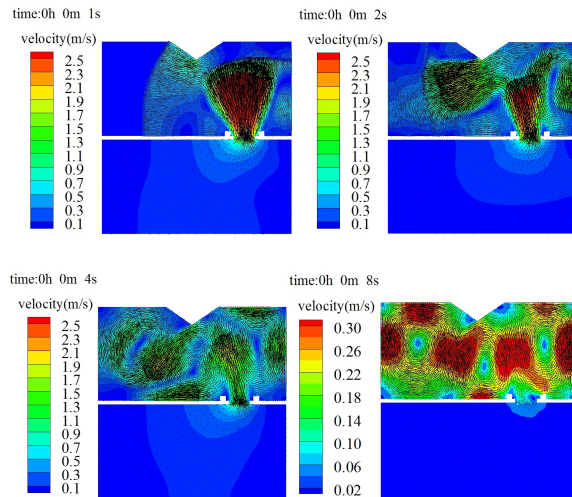
Figure 6. (c) Computed velocity fields of dambreak flow by using fully explicit scheme.
