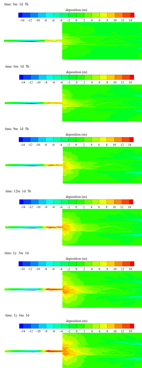
Figure 12. Long-term downstream sediment deposition contours.
