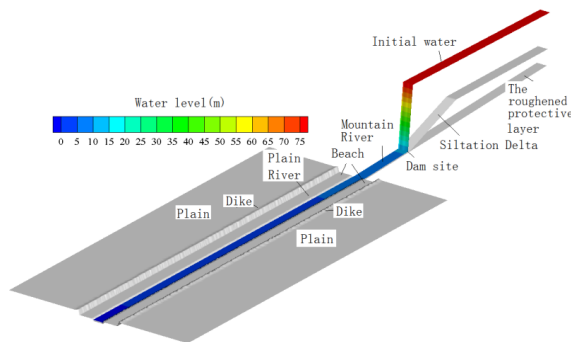
Figure 8. Schematic view of initial channel topography and reservoir area.
