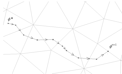
Figure 1. Schematic illustration of ELM tracking.
