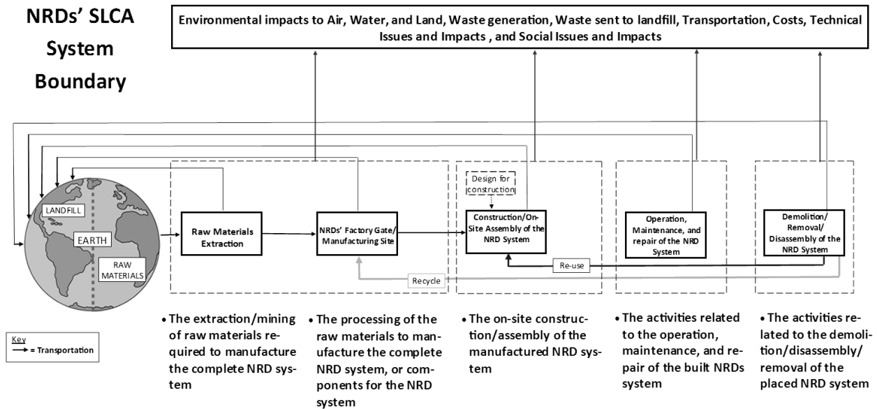
Figure 1: The NRDs' sustainability life cycle assessment (SLCA) system boundary (Source: Oltean-Dumbrava et al., 2016)
