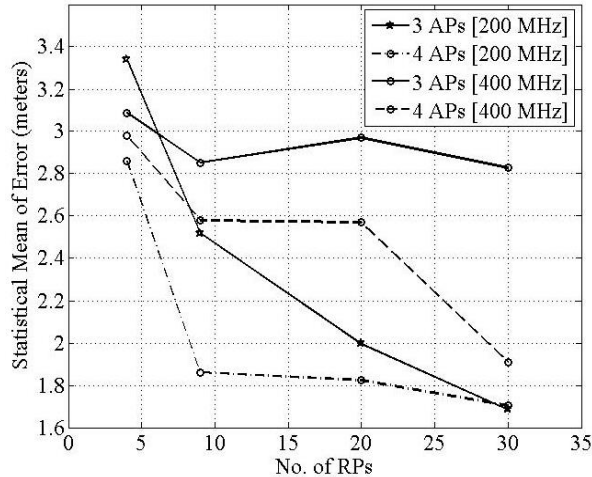
Fig. 7. Statistical mean error for the vector algorithm.
