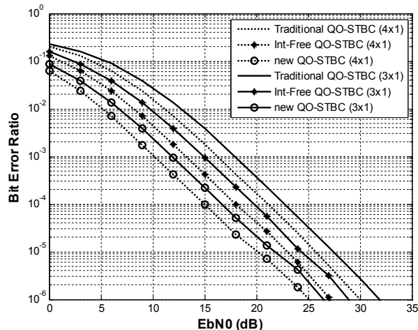
Figure 1: Comparison of new QO-STBC with traditional QO-STBC and interference-free QO-STBC
