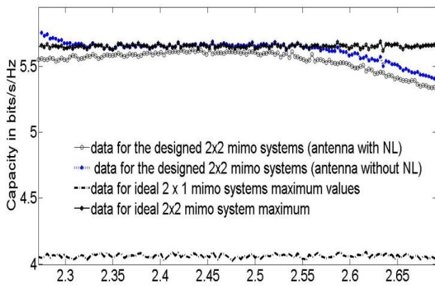
Figure 15. Simulated capacity of the proposed antenna with and without neutralization line.
