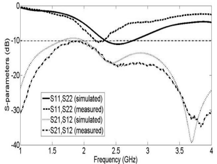
Figure 3. Comparative plot of s-parameters output for simulated and measured results for the proposed antenna without neutralization line.
