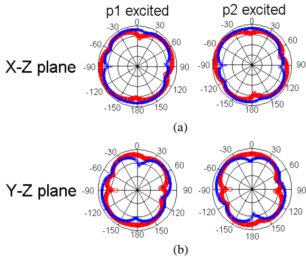
Figure 7. Simulated radiation patterns for the proposed antenna for two planes at 2.4 GHz; (a) X-Z plane. “xxxx” (blue) simulated cross-polarization, “oooo” (red) simulated co -polarization. (b) Y-Z plane. “xxxx” (blue) simulated co-polarization, “oooo” (red) simulated cross-polarization Port 1(left) excited and port 2(right) terminated in 50Ω.
