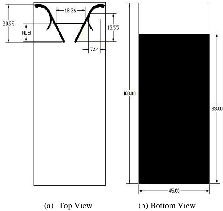
Figure 1. Geometry of the proposed antenna (in mm) (a) top view, and (b) Bottom view.
