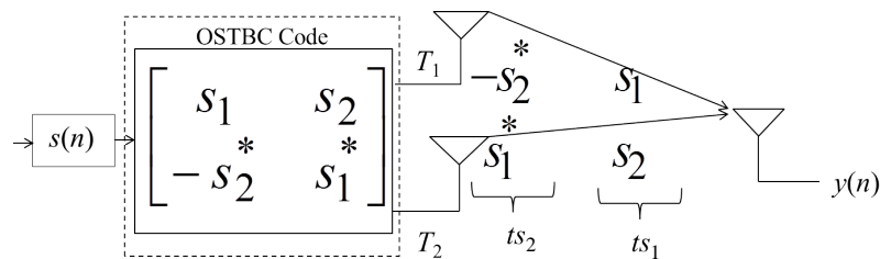
Figure 1. Architecture for implementation of OSTBC.
