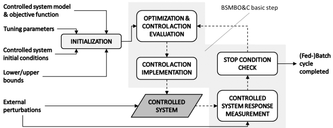
Figure 2. Simplified graphical description of the BSMBO&C algorithm
