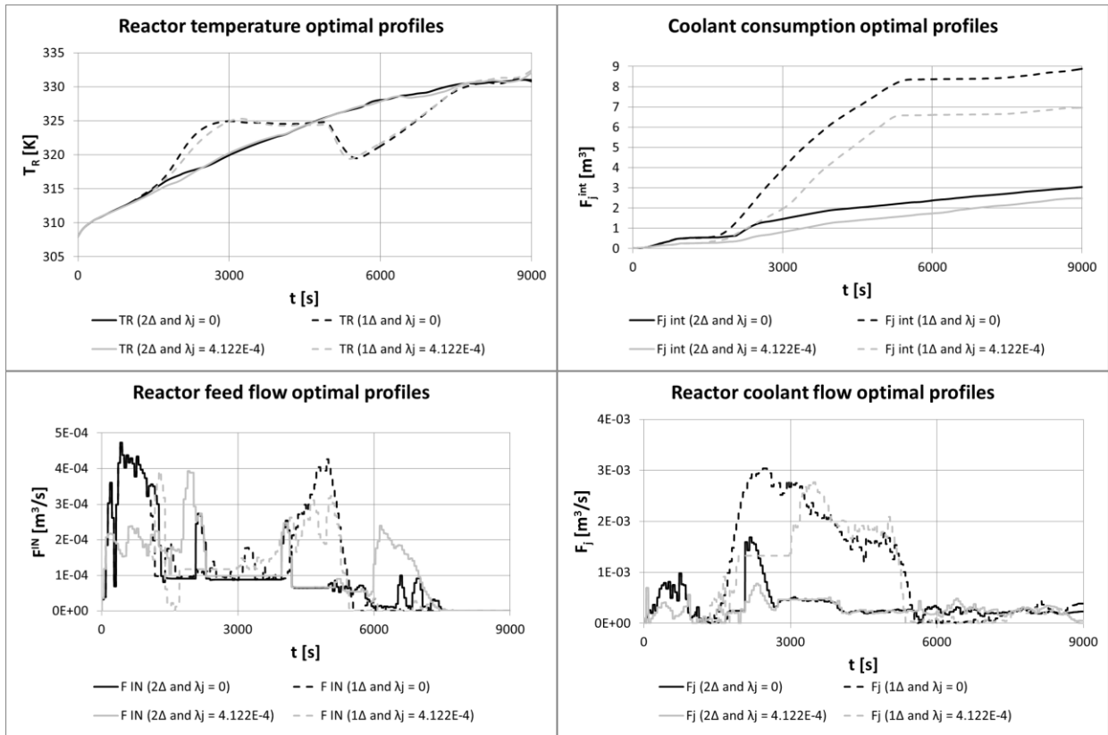
Figure 9. Williams-Otto fed-batch reactor optimal operation with ( \lambda_j \neq 0 ) and without ( \lambda_j = 0 ) the employment of the utilities-usage-related penalty terms approach ( U_{real} = 0.8875 \text{ kW/m}^2/\text{K} )
