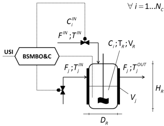
Figure 3. Williams-Otto fed-batch reactor layout (USI stands for user-supplied information)
