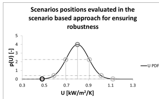
Figure 4. Graphical representation of the scenarios selection step output ( p(U) identifies the heat transfer coefficient probability density function (PDF) while the black, dark grey and light grey circles stand for worst case, nominal case and additional scenarios)
