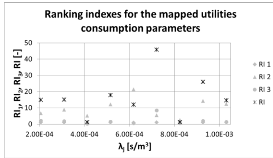
Figure 5. Trends of the ranking index and sub-indices for the only employed utility consumption parameter ( \lambda_j )
