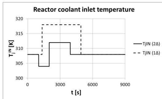
Figure 6. External perturbations imposed in the 2Δ and 1Δ cases
