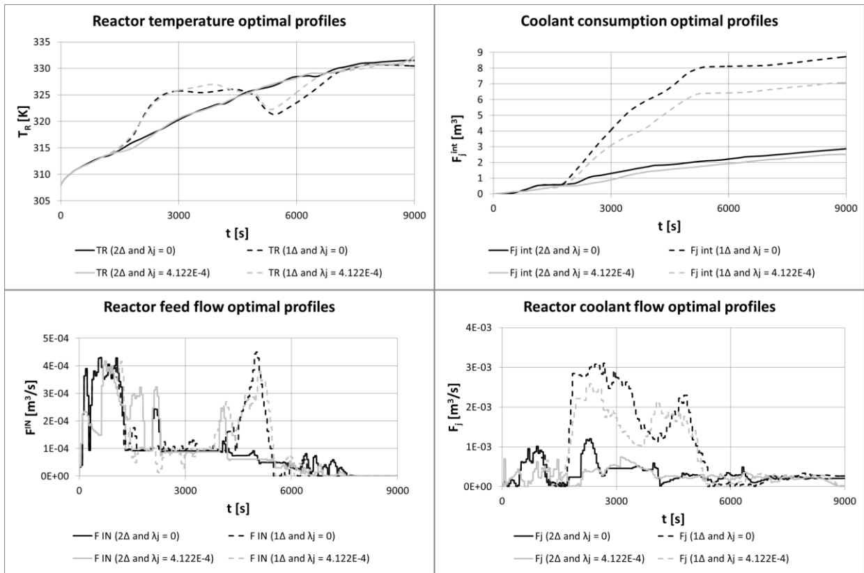
Figure 8. Williams-Otto fed-batch reactor optimal operation with ( \lambda_j \neq 0 ) and without ( \lambda_j = 0 ) the employment of the utilities-usage-related penalty terms approach ( U_{real} = 0.8 \text{ kW/m}^2/\text{K} )
