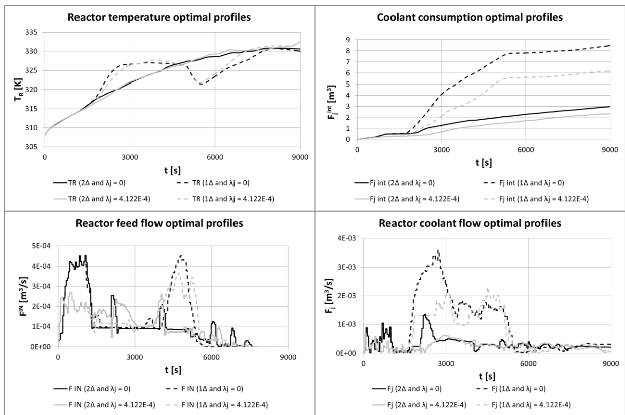
Figure 7. Williams-Otto fed-batch reactor optimal operation with ( \lambda_j \neq 0 ) and without ( \lambda_j = 0 ) the employment of the utilities-usage-related penalty terms approach ( U_{real} = 0.7125 \text{ kW/m}^2/\text{K} )
