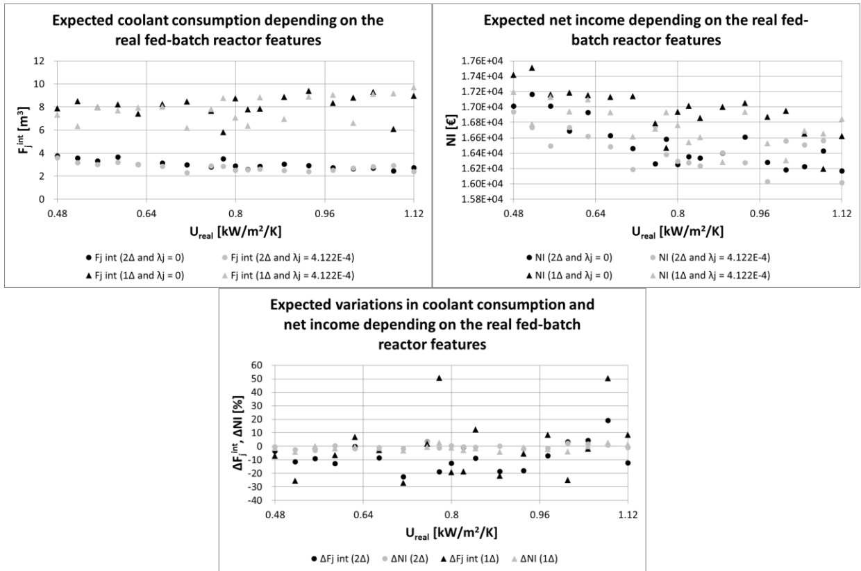
Figure 10. Effect of the employment of the utilities-usage-related penalty terms approach on the performance and sustainability in the optimal operation of the Williams-Otto fed-batch reactor
