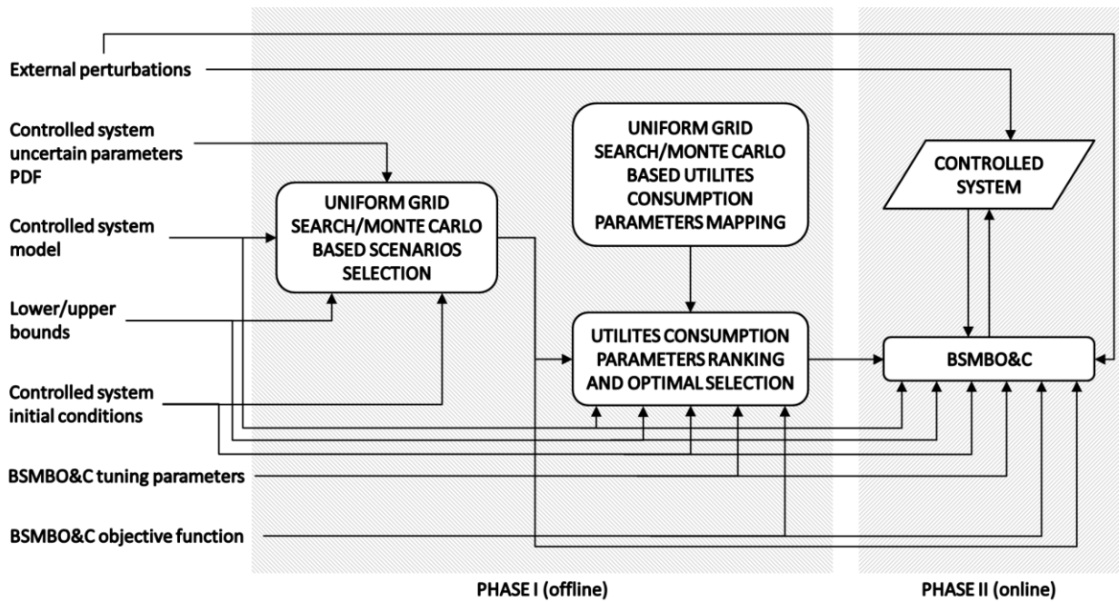
Figure 1. Schematic representation of the robust sustainable optimization & control strategy (RSOCS)
