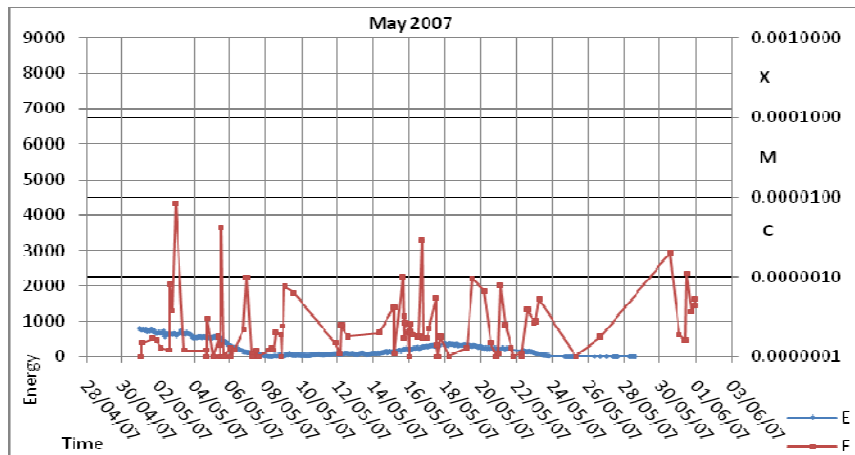
Figure 10. This plot shows the solar disk energy (Magnetic Complexity) and flares which occurred in May 2007.
