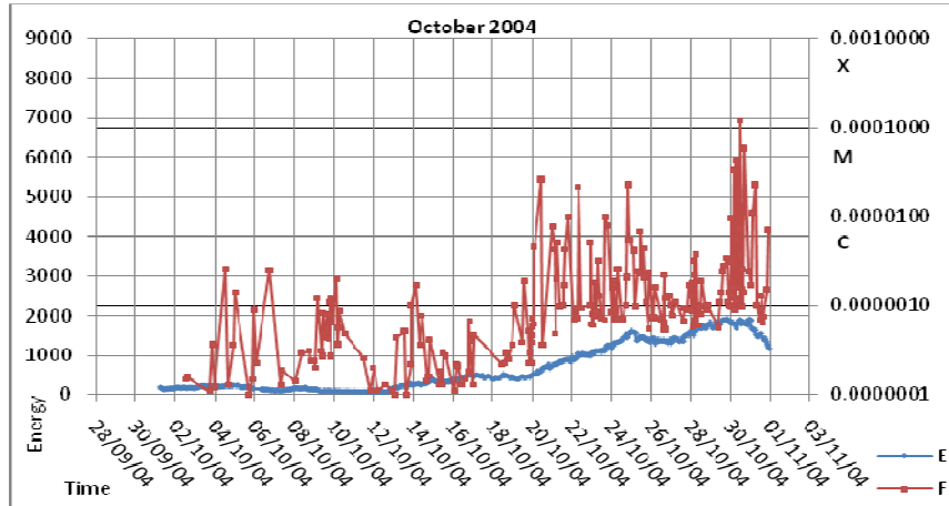
Figure 9. This plot shows the solar disk energy (Magnetic Complexity) and flares which occurred in October 2004.
