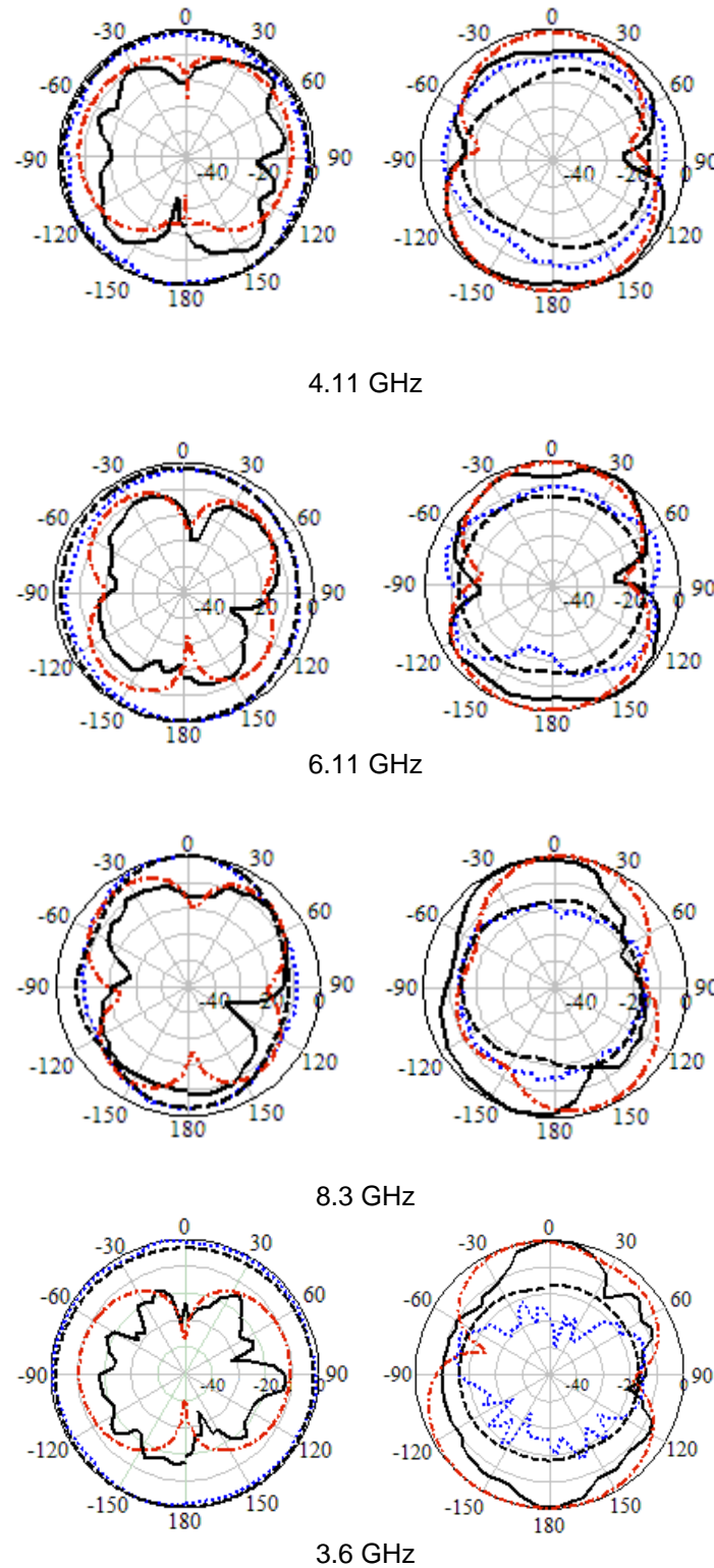
Fig. 12 Simulated and measured radiation patterns (a) in xz -plane and (b) in yz -plane. Simulated E_{\theta} : dashed-dotted line. Measured E_{\theta} : solid line. Simulated E_{\phi} : dashed line. Measured E_{\phi} : dotted line.
