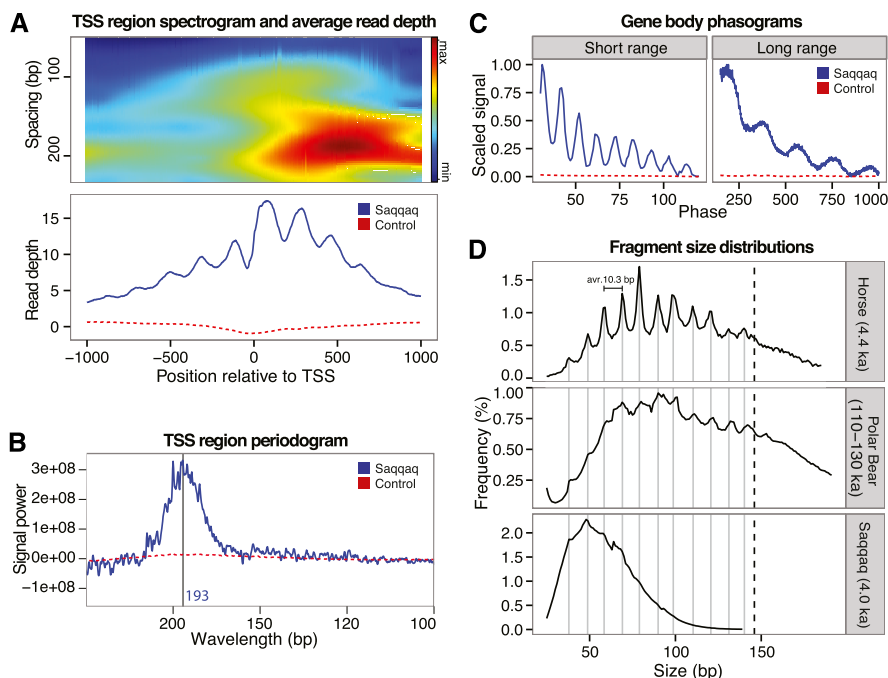
Figure 2. Read depth and fragment length periodicity. (A) Read-depth variation at TSS. Spectrogram around TSS ( top ) showing the strength of the periodicity signal at different wavelengths. Nucleosome abundance ( bottom ) summed over aligned transcription start sites. High occupancy at the +1 nucleosome position is characteristic of transcriptional activity. (B) Spectral density (periodogram) for TSS regions. The frequency spectrum shows a peak in relative signal at 193 bp corresponding to the expected inter-nucleosome distance. (C) 5' read-end phasograms showing the distribution of distances between reads in gene bodies. A clear \sim 200 -bp periodicity is apparent, consistent with the presence of nucleosomes ( right ). A short-range periodicity of \sim 10 bp is also apparent ( left ), corresponding to a turn of the DNA helix as it winds around the nucleosome. (D) Distribution of fragment sizes from ancient samples of horse ( top ), polar bear ( middle ), and Saqqaq ( bottom ) are consistent with preferential cleavage of exposed nucleosome-wrapped DNA strands every 10 bp.
