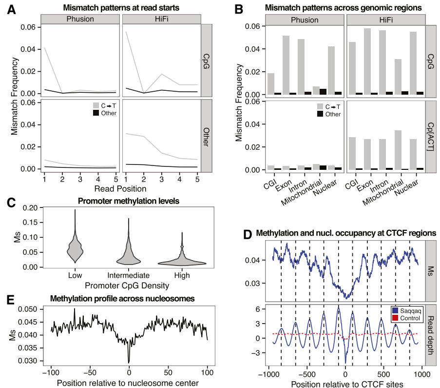
Figure 4. Substitution rates at CpG reveal methylation of DNA. (A) C→T mismatch rates (gray) versus rate of other mismatches (black) between a random subset of 1,000,000 Phusion (left) or HiFi (right) reads mapping uniquely. Reads are split by those starting with CpG (top; 26,864 Phusion and 25,568 HiFi reads) and other dinucleotides (bottom). (B) Mismatch frequencies for Phusion (left) and HiFi (right) for reads aligned to various genomic locations starting with the dinucleotides: CpG (top) and Cp[ACT] (bottom). (C) Distribution of M_s values for three classes of promoters with low, medium, and high CpG densities (Supplemental Material S13.2). (D) Methylation profile ( M_s , top) and read depth variation (bottom) at CTCF regions. Read depth provides a proxy for nucleosome occupancy. (E) Distribution of M_s values across nucleotide positions covered with nucleosomes, showing a depletion in methylation levels within a core region (20 nt before and after the nucleosome center) that is particularly marked at the nucleosome center.
