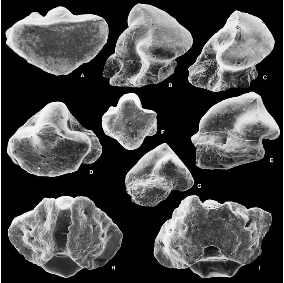
TEXT-FIG. 5. All specimens from lens between Wyke and Black Head siltstones unless stated otherwise. A–I, Spathobatis bugesiacus Thiolliere, 1854. A–B, P. 65709, lateral tooth of female, width 0.8 mm; \times 70 . 1, occlusal view. 2, oblique lateral view. C, P. 65710, lateral tooth of male, oblique lateral view, width 0.6 mm; \times 85 . D–E, P. 65705, anterior tooth of male, width 0.8 mm; \times 55 . D, occlusal view. E, lateral view. F–G, P. 65706, extreme anterior tooth, width 0.5 mm; \times 55 . F, occlusal view. G, lateral view. H, P. 65707, tooth with open nutritive groove, Small Mouth Sands, width 0.9 mm; \times 62.5 . I, P. 65708, tooth with closed nutritive groove, Small Mouth Sands, width 1 mm; \times 62.5 .
