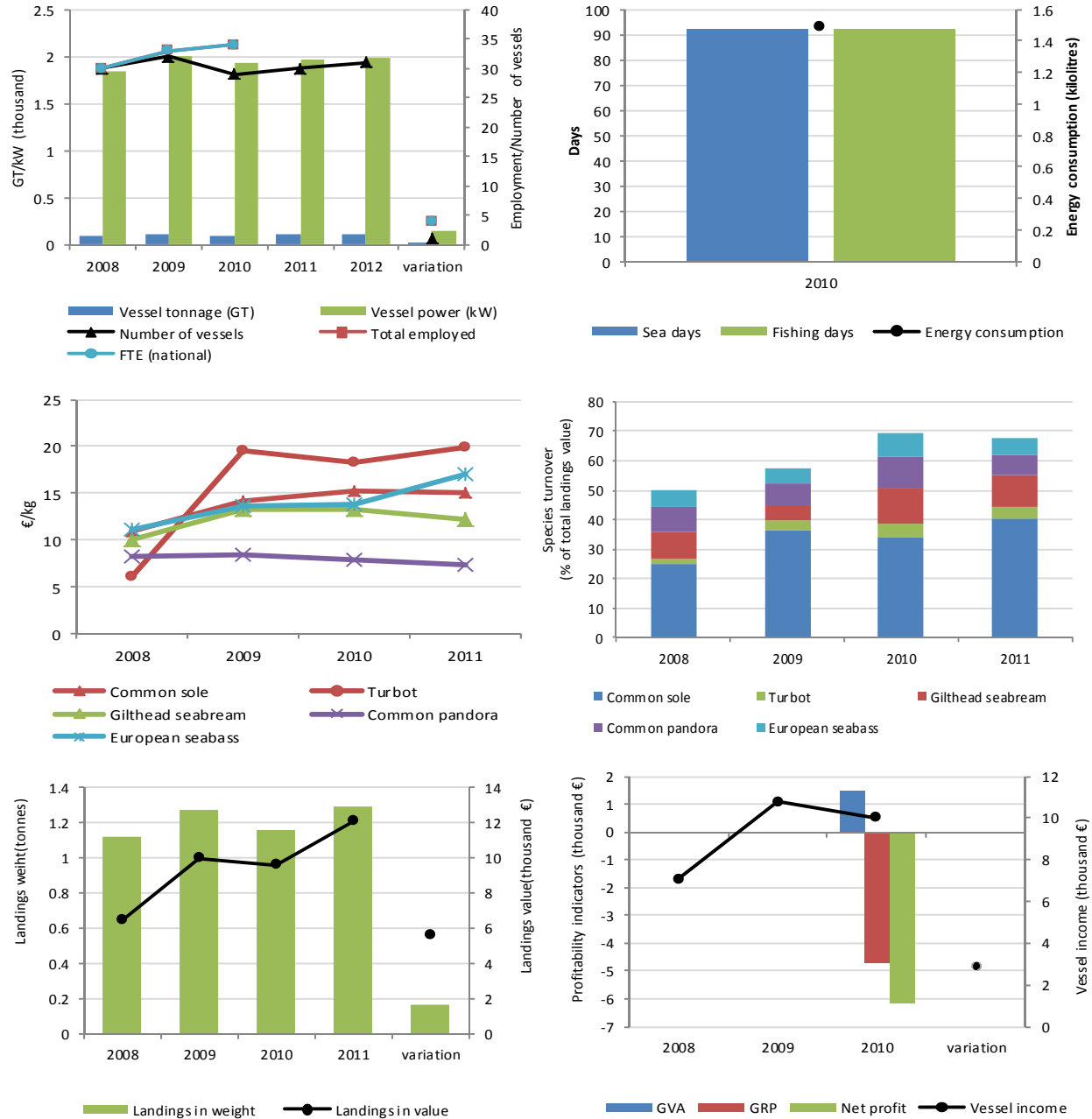
Figure 5.19.6 Key indicators for the average vessel in the Slovenian DFN VL0612 fleet segment, 2008-2011:
