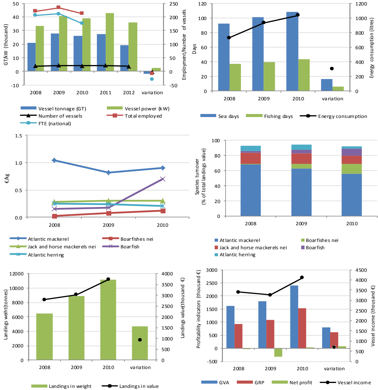
Figure 5.10.6 Key indicators for the average vessel in the Irish TM VL40XX fleet segment, 2008-2012: top left – fleet capacity and employment; top right – fishing activity and effort; middle left – average prices (€/kg) for key species; middle right - turnover as a percentage of total value of landings for key species; bottom left - landings in value and weight; bottom right –main economic indicators for the average vessel (variation 2010-2008)
