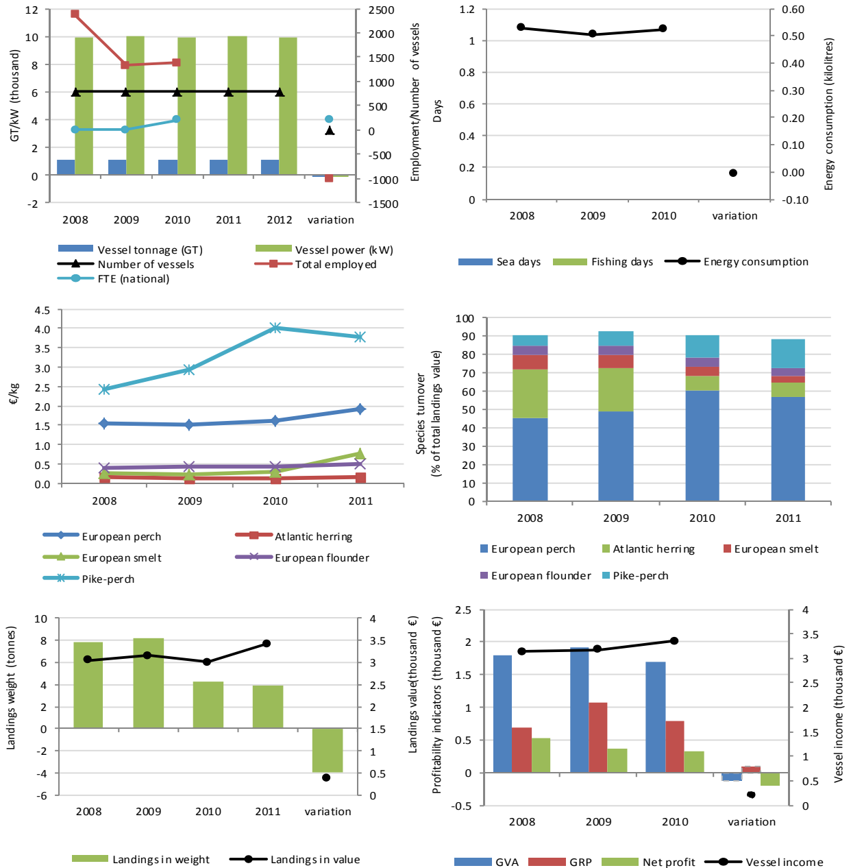
Figure 5.5.7 Key indicators for the average vessel in the Estonia PG VL0010 fleet segment 2008-2011:
