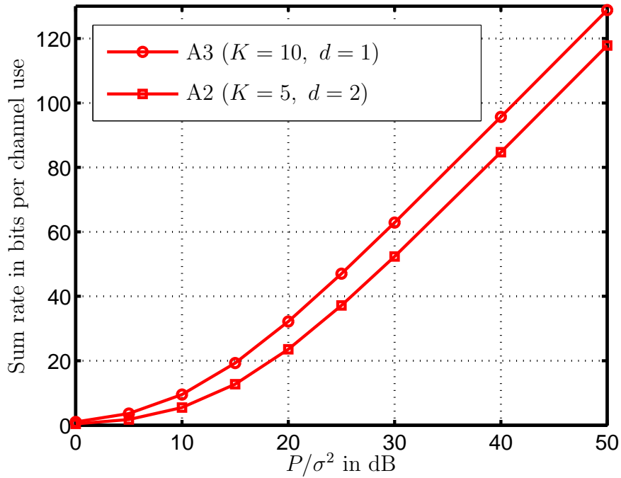
Figure 3.3. Sum rate for the proposed IA algorithm for different number of node pairs and data streams
