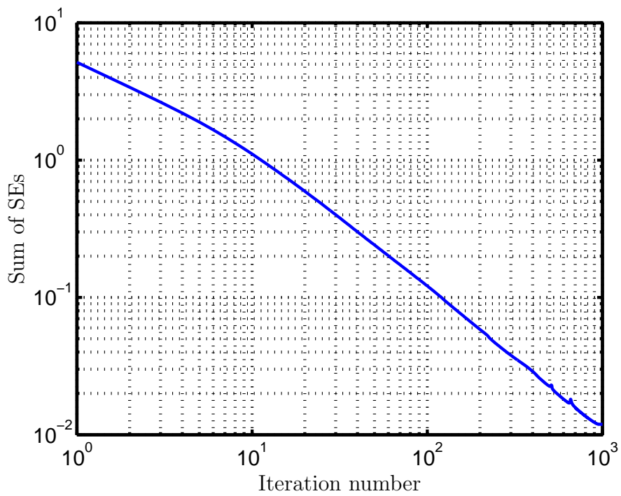
Figure 4.7. Average of the sum of SEs of different channel realizations versus the iteration number in scenario C4 with normalization of the variables
