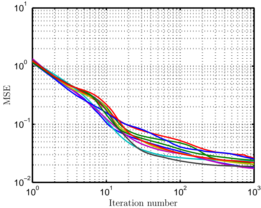
Figure 5.8. MSE versus the iteration number in scenario B4
