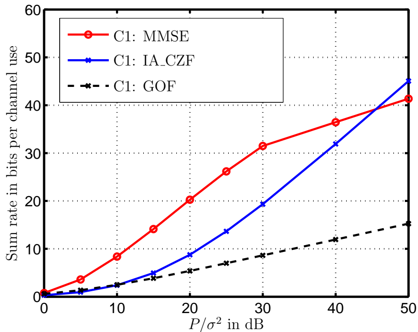
Figure 5.5. Sum rate performance of the MMSE, the IA_CZF, and the reference GOF algorithms versus P/\sigma^2 for scenario C1
