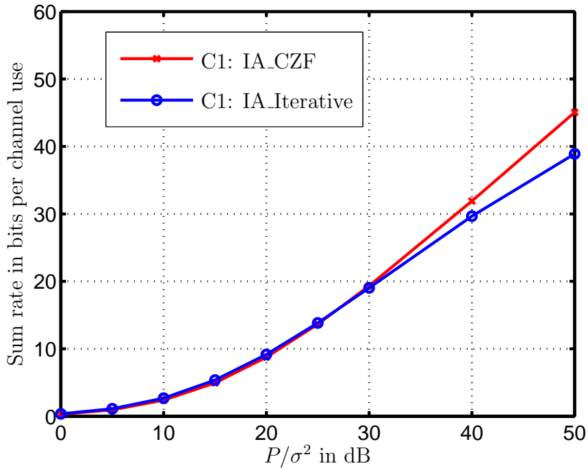
Figure 4.3. Sum rate performance of the IA_CZF and the IA_Iterative algorithms versus P/\sigma^2 for scenario C1
