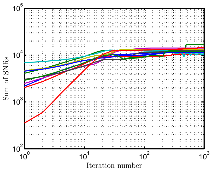
Figure 5.7. Sum of SNRs versus the iteration number in scenario B4 with normalization of the variables
