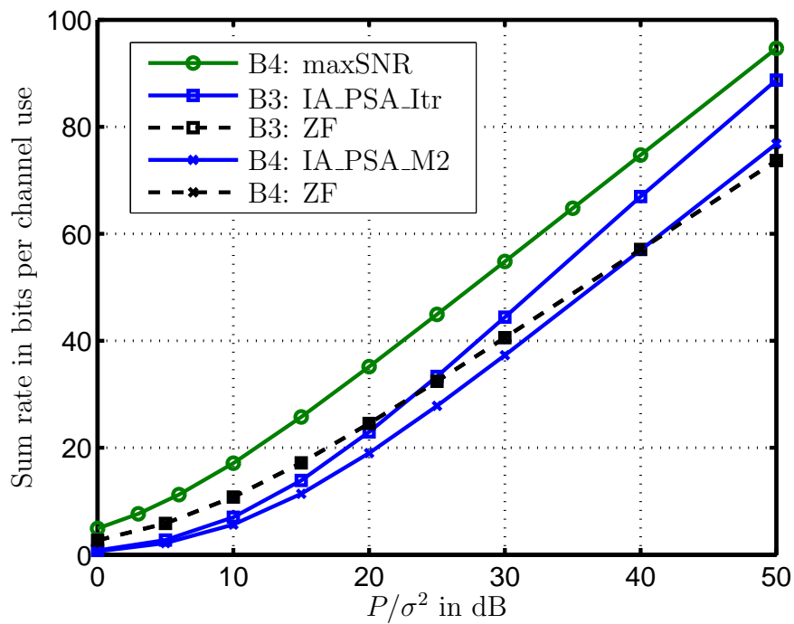
Figure 5.3. Sum rate performance of the maxSNR, the IA_PSA_Itr, the IA_PSA_M2, and the reference ZF algorithms versus P/\sigma^2 for scenarios B3 and B4
