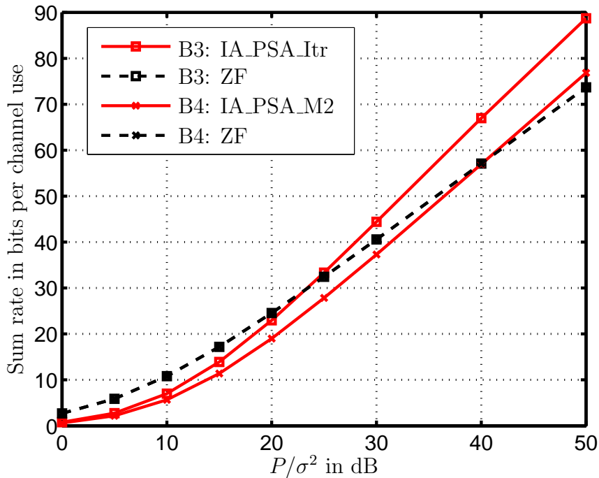
Figure 3.7. Sum rate performance of the IA_PSA_Itr, the IA_PSA_M2 and the reference ZF algorithms versus P/\sigma^2 for scenarios B3 and B4
