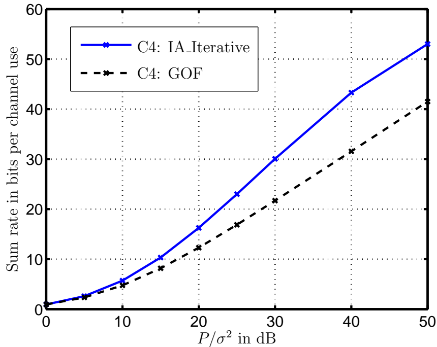
Figure 4.4. Sum rate performance of the IA_CZF algorithm and the reference GOF algorithm versus P/\sigma^2 for scenario C4
