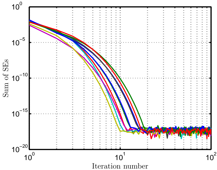
Figure 4.5. Sum of SEs versus the iteration number in scenario C1
