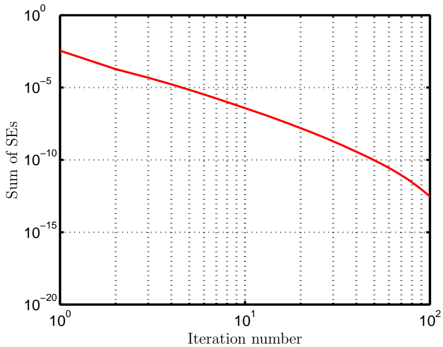
Figure 4.6. Average of the sum of SEs of different channel realizations versus the iteration number in scenario C1
