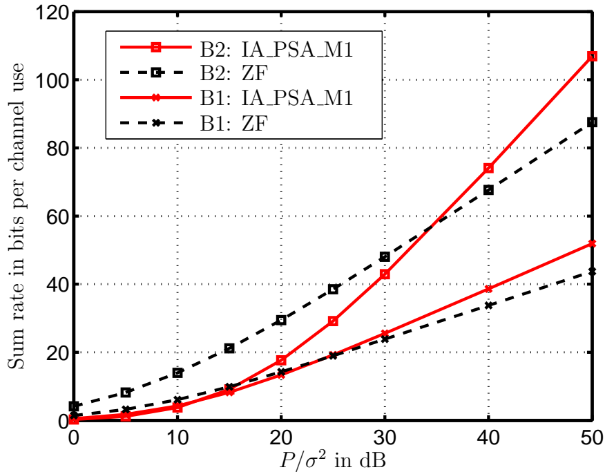
Figure 3.6. Sum rate performance of the IA_PSA_M1 algorithm and the reference ZF algorithm versus P/\sigma^2 for scenarios B1 and B2
