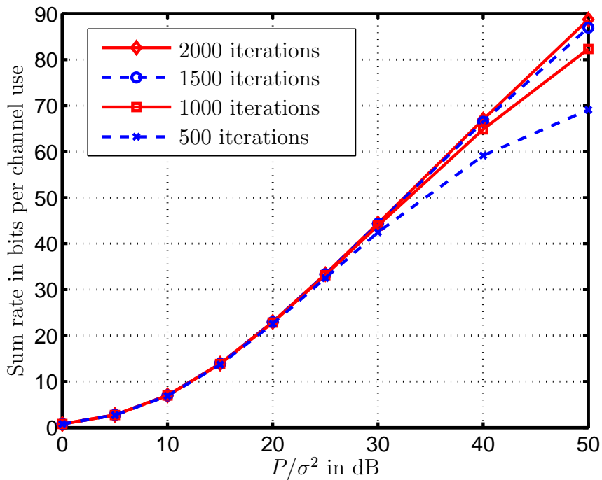
Figure 3.8. Sum rate comparison with different number of iterations for scenario B3
