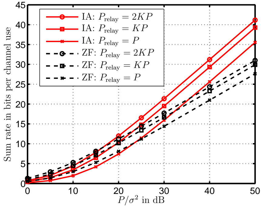
Figure 3.2. Influence of the relay power P_{\text{relay}} on the sum rate performance versus P/\sigma^2 for the proposed IA algorithm and the reference ZF algorithm in Scenario A1
