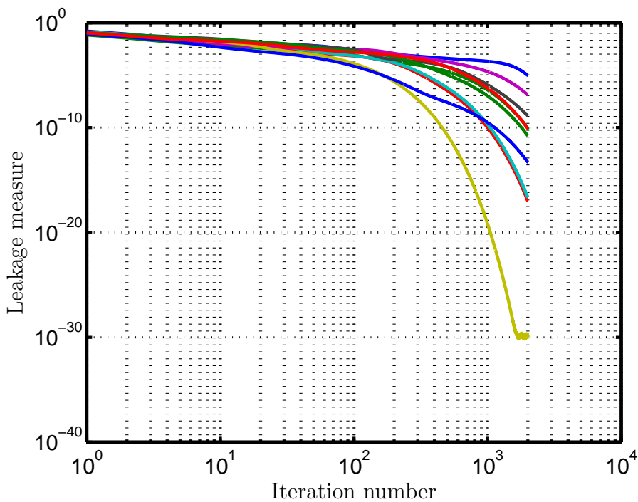
Figure 3.9. Leakage measure of IA_PSA_Itr versus number of iterations in B3
