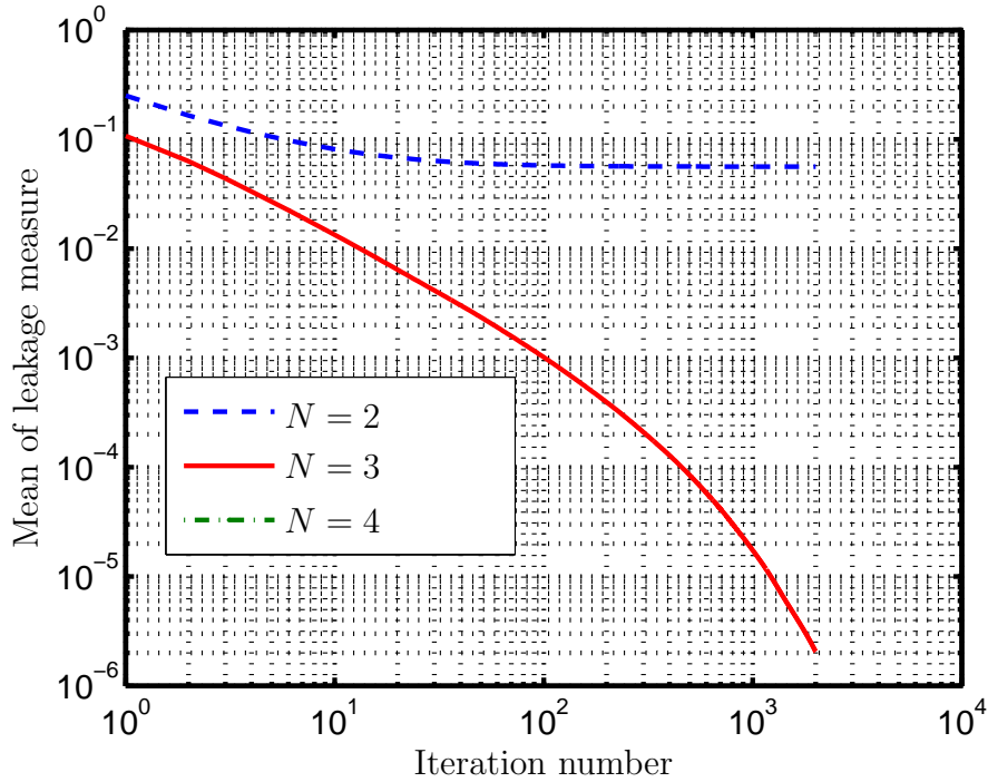
Figure 3.11. mean of the leakage measure versus the iteration number for the IA-PSA_Itr for different number N of antennas at the nodes
