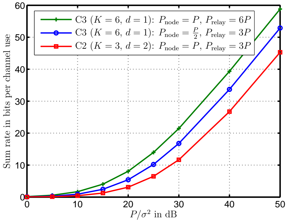
Figure 4.2. Influence of d , K , and the maximum transmit power at the nodes and at the relays on the sum rate in scenario C2 and in scenario C3 for a fixed number of DoF
