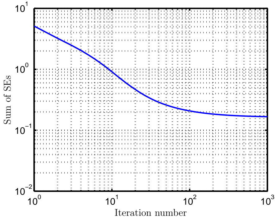
Figure 4.8. Average of the sum of SEs of different channel realizations versus the iteration number in scenario C4 without normalization of the variables
