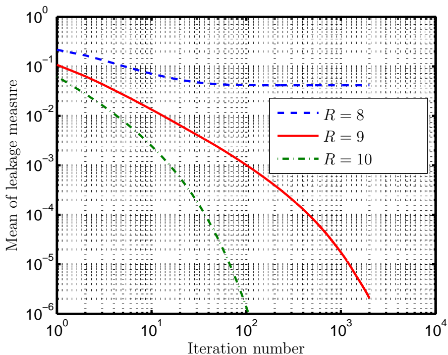
Figure 3.10. Mean of the leakage measure versus the iteration number for the IA-PSA_Itr for different number R of antennas at the relay
