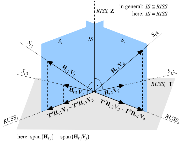
Figure 3.5. Illustration of PSA for N = 1 , d = 1 , R = 3 , and K = 2
