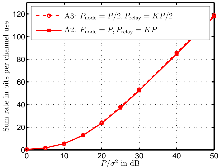
Figure 3.4. Sum rate for the proposed IA algorithm for different number of node pairs and data streams with the same total power in scenario A2 and in scenario A3
