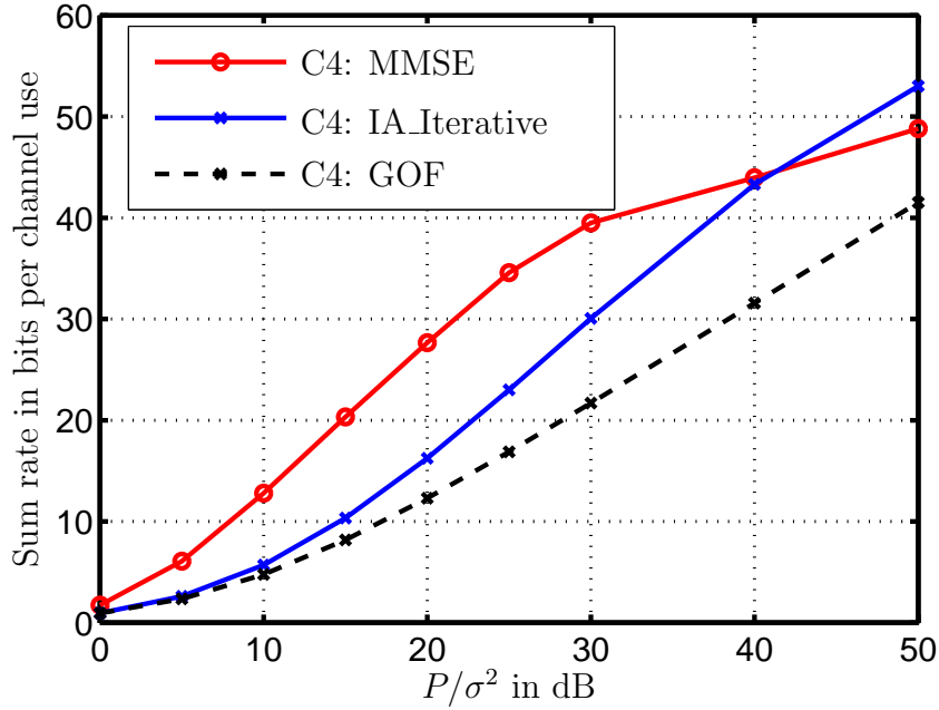
Figure 5.6. Sum rate performance of the MMSE, the IA.Iterative, and the reference GOF algorithms versus P/\sigma^2 for scenario C4
