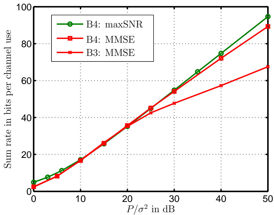
Figure 5.4. Sum rate performance of the maxSNR and the MMSE algorithms versus P/\sigma^2 for scenarios B3 and B4
