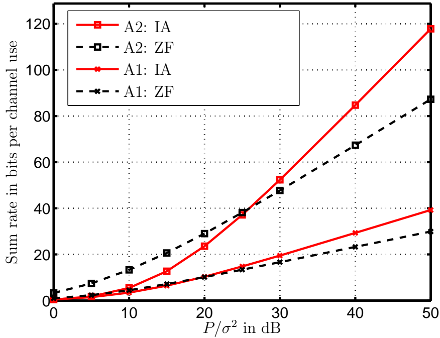
Figure 3.1. Sum rate performance of the proposed IA algorithm and the reference ZF algorithm versus P/\sigma^2 for scenarios A1 and A2
