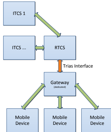
Figure 1: System concept of IP-KOM-OeV
