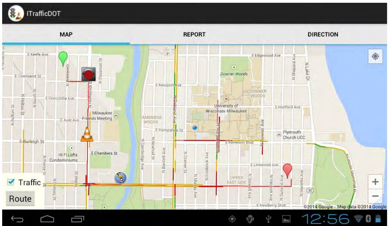
Figure 5.10. Warning messages of incident events customized to the selected route
