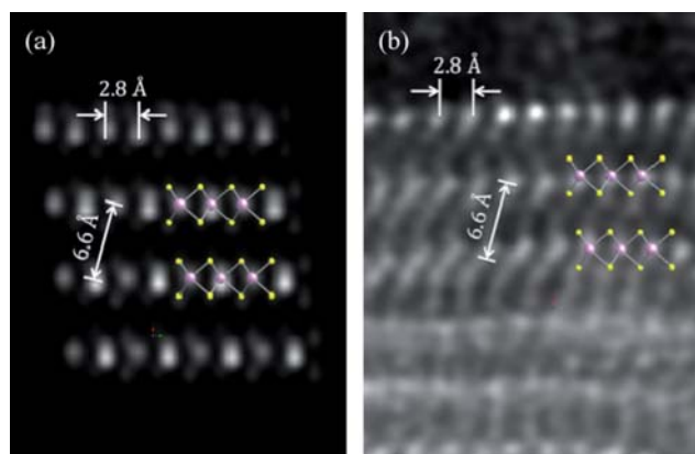
Fig. 6 (a) STEM simulated image of a segment of the multiwall tube model presented in Fig. 6. The resolution and contrast are high enough to identify the S columns, as can be noted by the superposition of the ball and stick model (pink balls: Mo atoms; yellow balls: S atoms). Measurements were made directly on the STEM simulated image. (b) Segment of an aberration-corrected STEM micrograph, where the S columns are also identifiable. [Note that the distances between the Mo–Mo atoms is 2.8 Å and the distance between the layers correspond to 6.6 Å].
