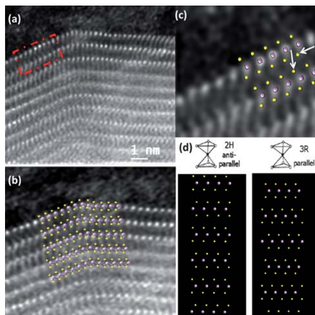
Fig. 9 (a) Aberration-corrected STEM-HAADF images of a MoS 2 nanotube. The atomic resolution image of the area marked by a dash square in (a) is shown in (b) and (c) Detailed atomic distribution of the Mo and S atoms forming the layers with a projected model on top, (d) Structural models of MoS 2 showing the 2H and the 3R modifications.
