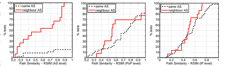
Figure 6. DisNETPerf approach. DisNETPerf achieves almost perfect path similarity at the AS level when IP_{DNP} is located in the same AS of IP_s , and path similarity above 50% for most of the cases, also at the PoP and interface level.
