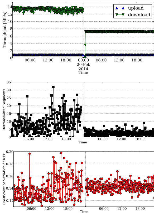
Figure 2. Evolution of time of the throughput measured by one active probe (top), the number retransmitted segments (center), and the coefficient of variation of the RTT (bottom). U-1Mbps/D-16Mbps ADSL probe.
