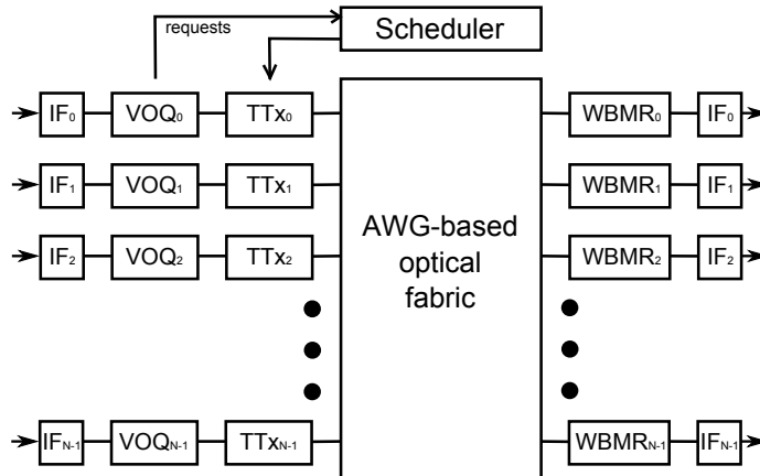
Figure 1: Switch Architecture
