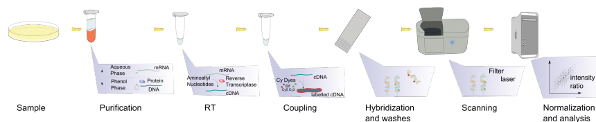
Figure 14: Steps required in a microarray experiment
