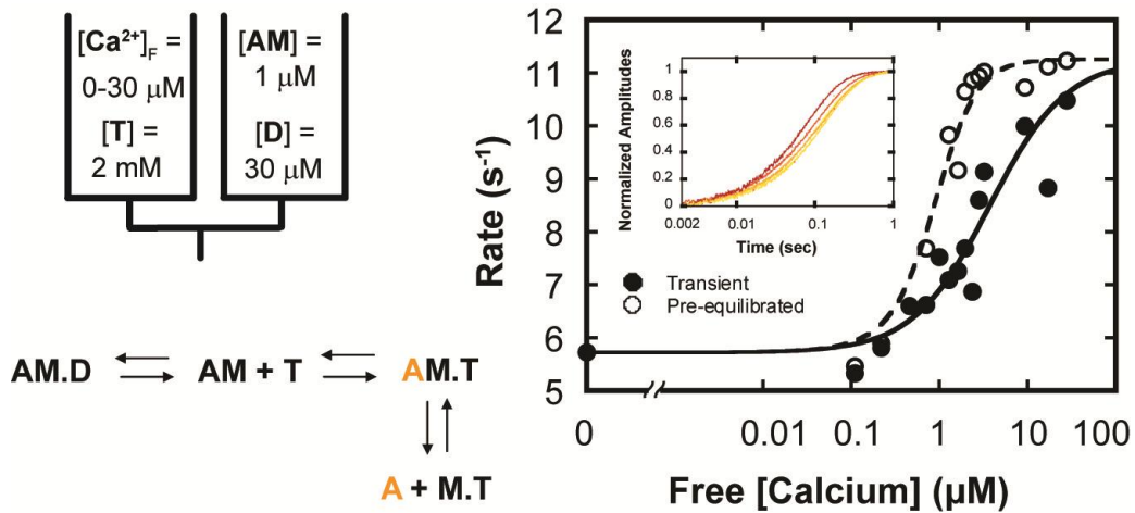
Figure 2.21 - Calcium-dependent increase in the ADP Release Rate k_{+5}' for myo1b IQ is rapid.
