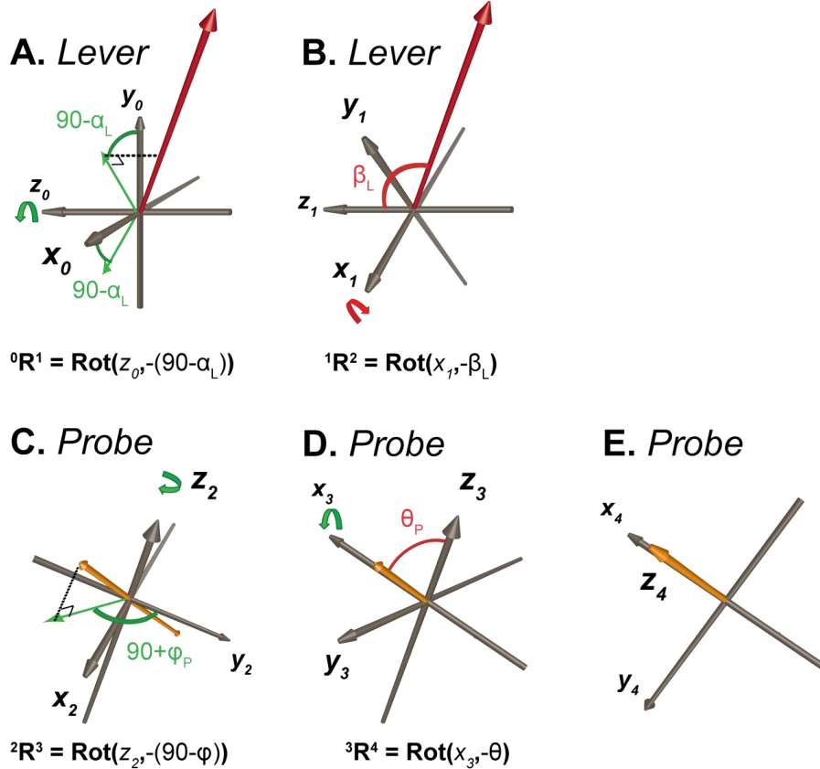
Figure 5.5 – Rotation Scheme.
