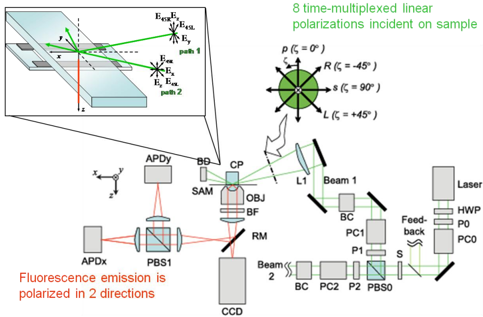
Figure 3.1 - Experimental Setup for polTIRF Microscopy.
