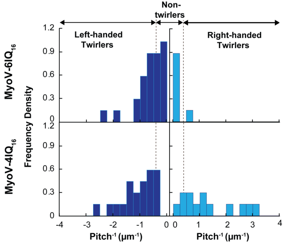
Figure 3.17 – Inverse pitch ( \mu\text{m}^{-1} ) distributions for \text{myoV-6IQ}_{16} and -4\text{IQ}_{16} .
