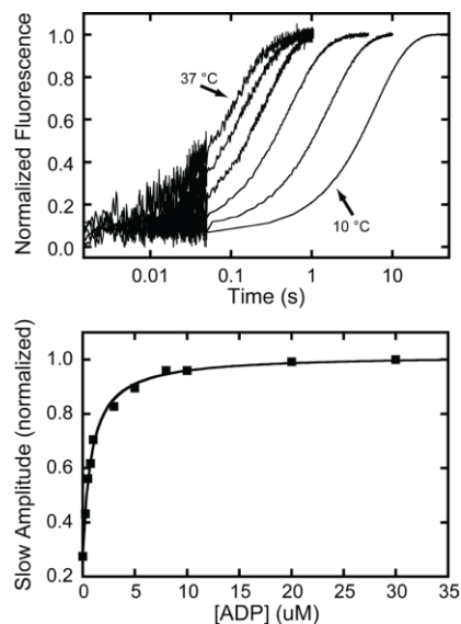
Figure 2.8 - ADP release from actomyo1b IQ .
