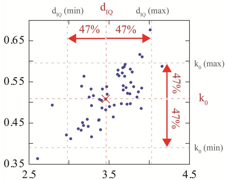
Figure 5.2 – Calculating the confidence interval
