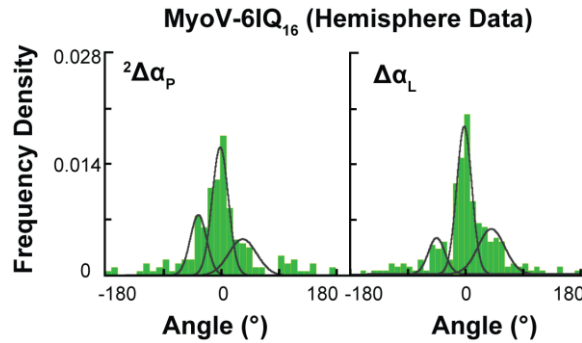
Figure 3.12 – Distribution of {}^2\Delta\alpha_P and \Delta\alpha_L for myoV-6IQ 16 with probe solution isolated to a hemisphere of space.
