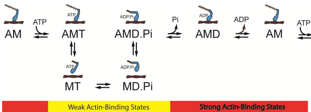
Figure 1.2 – Myosin crossbridge cycle
