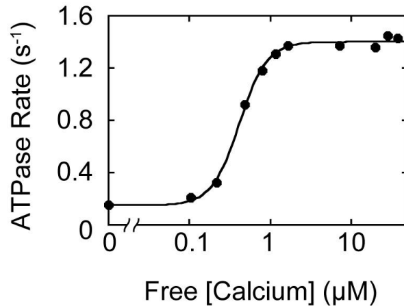
Figure 2.12 - The Steady State ATPase Rates for Myosin-Ib are Highly Sensitive to Calcium Concentration.
