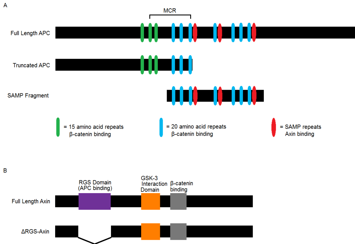
Figure 1-2. Domain structure of APC and Axin. (A) The mutation cluster region (MCR) within APC is immediately N-terminal to the first Axin binding SAMP repeat. Oncogenic Apc mutations truncate within the MCR, removing the SAMP repeats and abolishing direct interaction with Axin. An example of a fragment containing the SAMP repeats (SAMP fragment) that rescues aberrant Wnt signaling in Apc mutant colorectal cancer cells is also shown. (B) Full length Axin binds APC, GSK-3 and β-catenin through distinct domains. ΔRGS-Axin lacks the APC binding domain and therefore cannot directly interact with APC.
