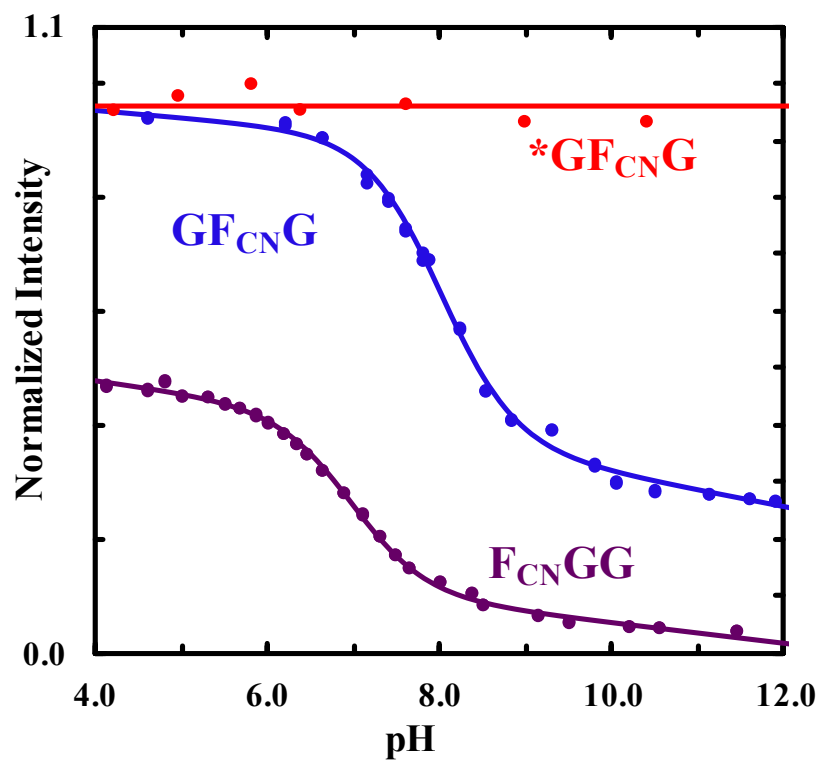
Figure 3.2 Normalized Phe CN fluorescence intensity versus pH of three tripeptides, as indicated. In each case, the smooth line represents the best fit of the corresponding fluorescence titration curve to Equation 3.1 and the resulting pK_a value is listed in Table 3.1.
