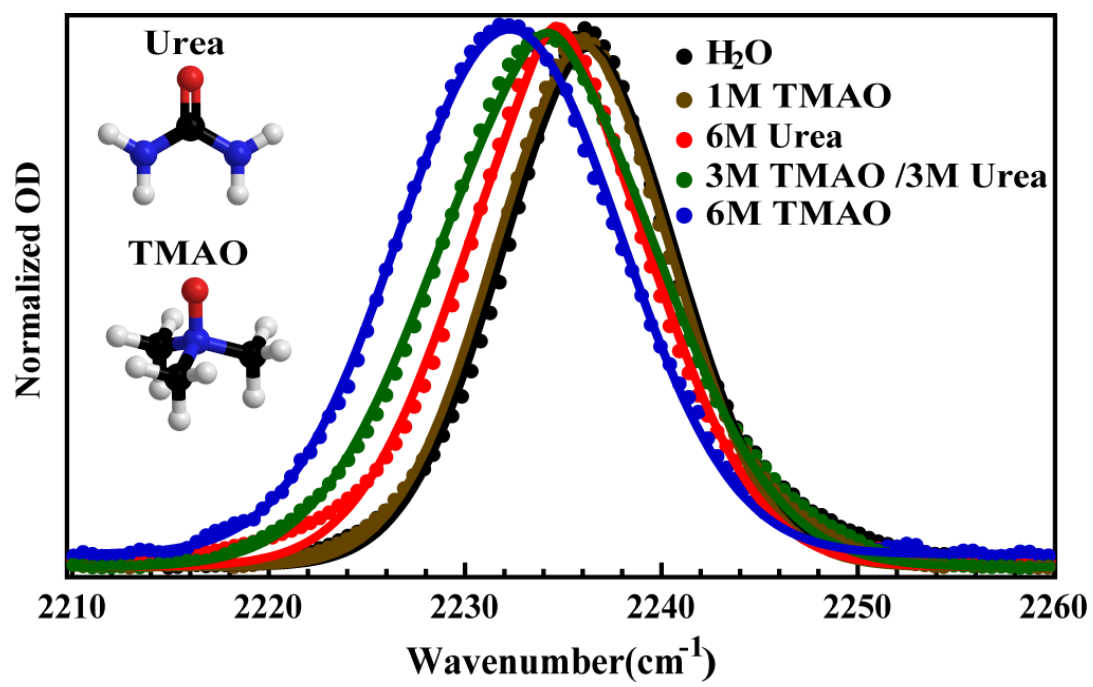
Figure 5.1 The C \equiv N stretch bands of GF CN G obtained under different solvent conditions, as indicated. The solid lines are fits of these spectra to the linear response function using Equation 5.2 to Equation 5.4 in the text and the resulting fitting parameters are listed in Table 5.1. The structures of urea and TMAO are shown as insets.
