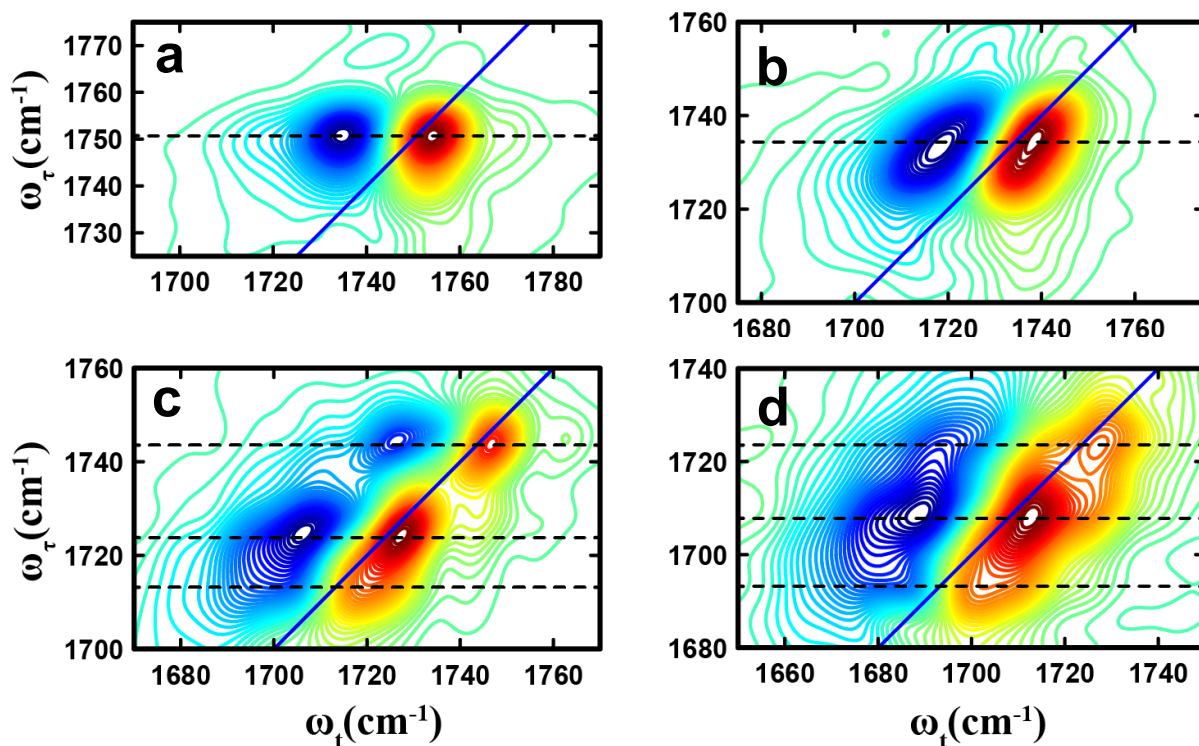
Figure 6.4 2D IR spectra of MP in a) hexane, b) DMSO, c) methanol, and d) water collected at zero waiting time (T). It is clear that for MP in hexane and DMSO, there is only one resolvable peak, consistent with the linear IR measurements. Similarly, the 2D IR spectrum in methanol, which consists of three peaks, is also in agreement with the FTIR spectrum. On the other hand, there are three peaks found in the 2D spectrum of MP in water. While the two stronger peaks at higher frequencies coincide with those observed in the linear IR spectrum, the low frequency transition is due to MP dimerization and thus is not discussed in the text.
