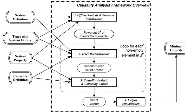
Fig. 3. Causality Analysis Framework Overview
