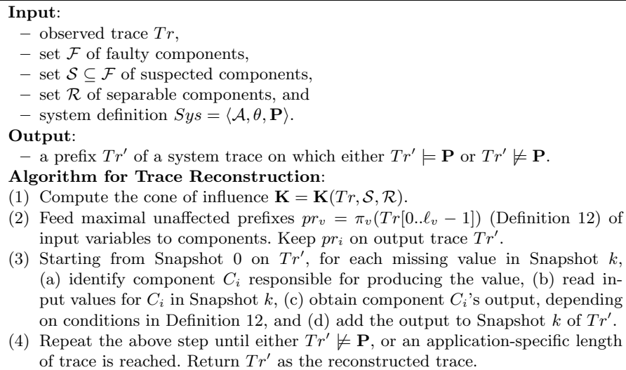
Fig. 4. Trace Reconstruction Algorithm
