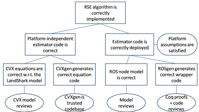
Figure 6. Argument for the code-level claims
