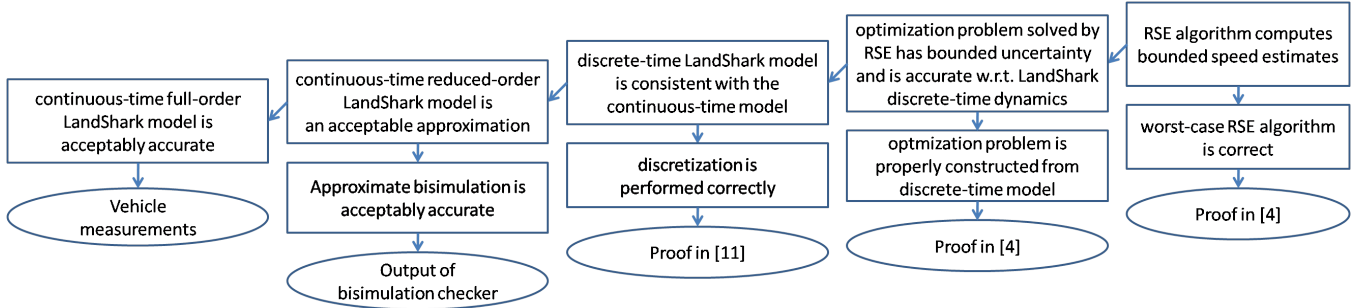
Figure 5. Control-level reasoning
