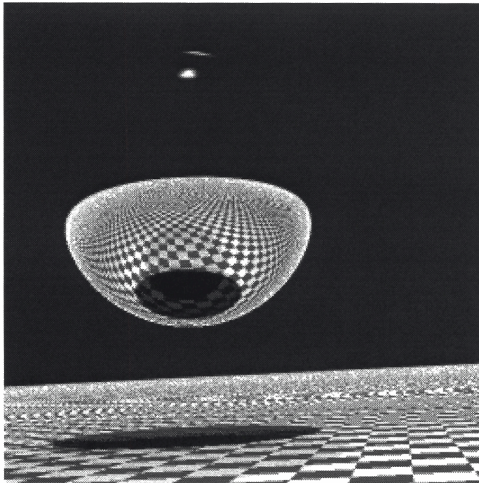
Figure 12: Test Scene 1 with CMAM off
