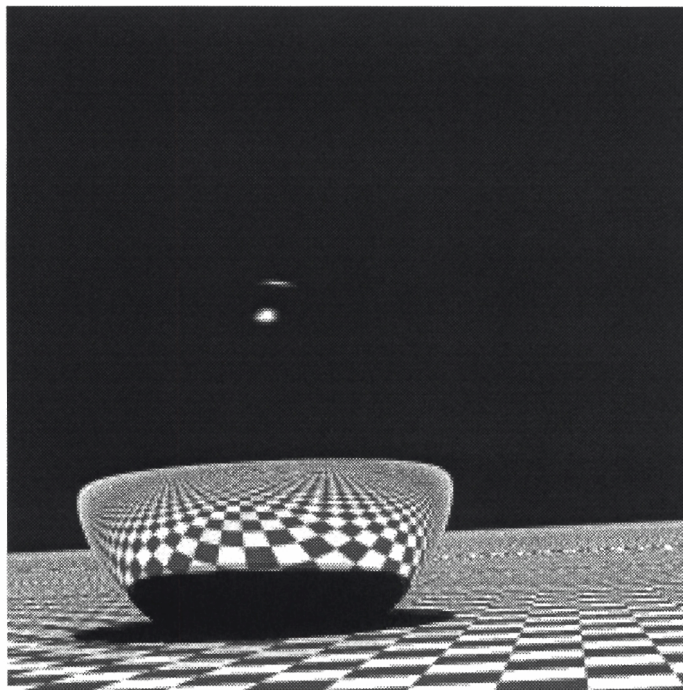
Figure 13: Test Scene 2 with CMAM on
