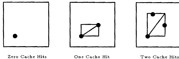
Figure 8: MIP Map Approximation Using the CMAM
