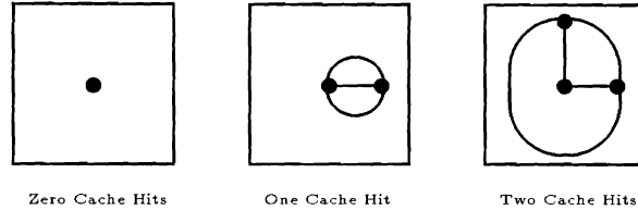
Figure 10: EWA Approximation Using the CMAM
