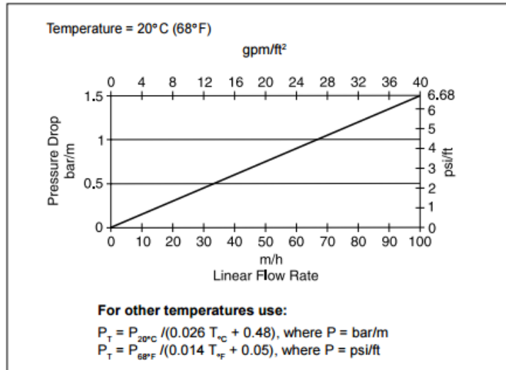
Figure 2. Pressure drop
