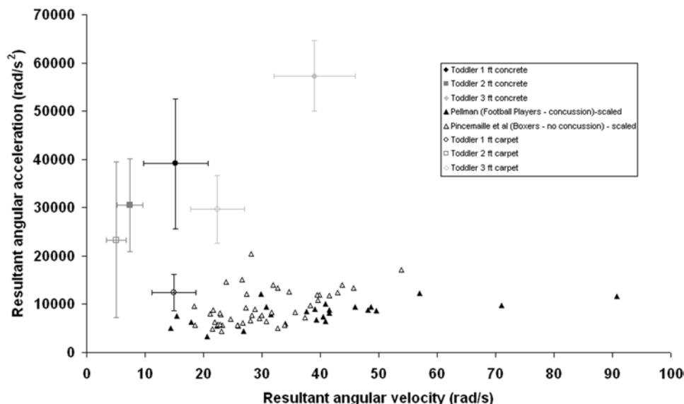
Fig. 9. Resultant acceleration/velocity data from toddler drops compared with mass scaled concussion data from boxers and football players.
