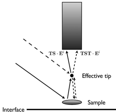
(b) Model of the tip
