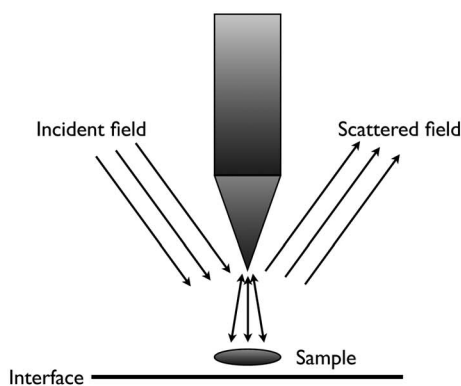
(a) Apertureless NSOT
