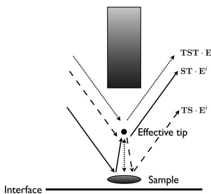
(b) Model of the apertureless tip
