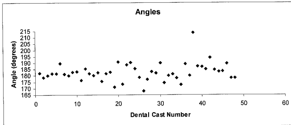
Graph 2: Angle Dispersal
