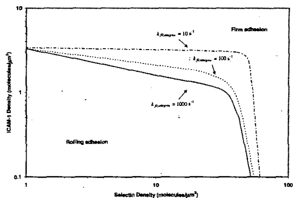
Fig. 1. The state diagram for adhesion mediated by two receptors. For each rolling state, the boundary represents a mean velocity of 0.02V_H .
