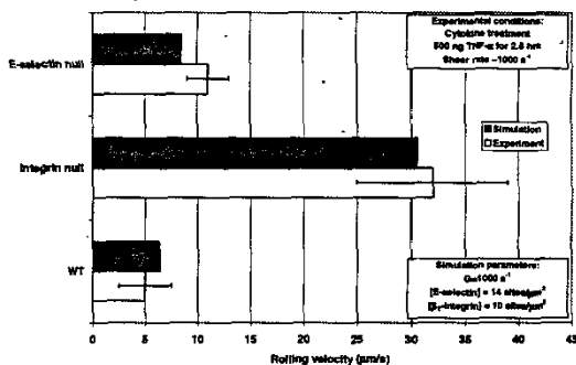
Fig. 2. Comparison of two-receptor adhesive dynamic simulations to experimental data from Kunkel and coworkers [11]. This calculation is performed at k_{f, \text{integrin}}^0 = 1000 \text{ s}^{-1} .
