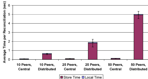
Figure 12: The effect on execution time when the number of peers is increased.
