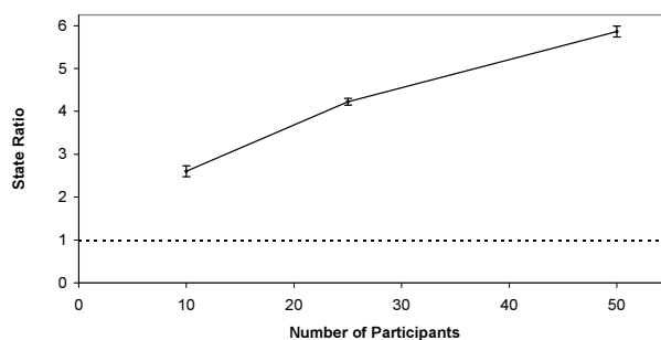
Figure 11: The change in state ratio when the number of peers is increased.
