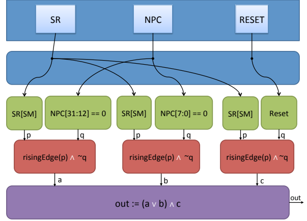
Figure 5: Fabric configured with a macro assertion that detects incorrect privilege escalations.
