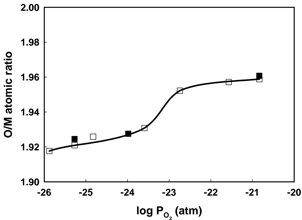
Figure 7a). O/M ratios as a function of P(\text{O}_2) for (\square)\text{Ce}_{0.14}\text{Zr}_{0.86}\text{O}_2 sample after calcination for 4 hours at 973 K ( \square ) and 1323 K ( \blacksquare ).
