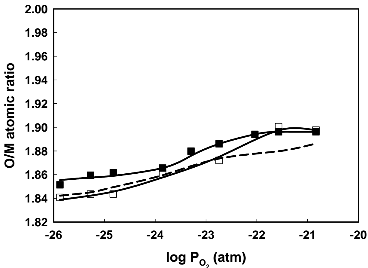
Figure 7c). O/M ratios as a function of P(O_2) for the Ce_{0.33}Zr_{0.67}O_2 sample after calcination for 4 hours at 973 K (□) and 1323 K (■). The simulated result (---) was calculated by assuming the sample calcined to 1323 K could be modeled as a physical mixture of Ce_{0.81}Zr_{0.19}O_2 and Ce_{0.25}Zr_{0.75}O_2 .
