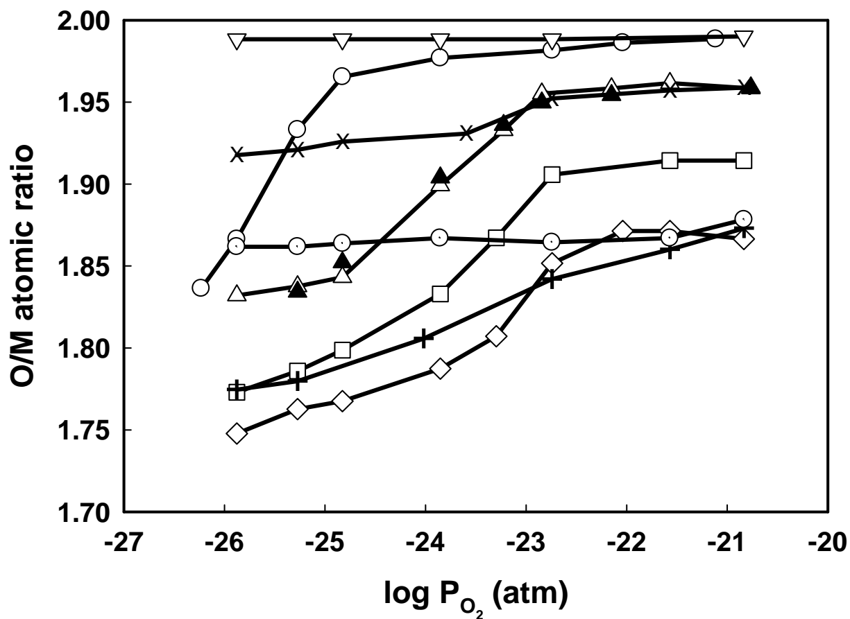
Figure 3. Oxygen to total metal (Ce+Zr) ratios for the Ce_yZr_{1-y}O_{2-x} samples, following calcination at 973 K, as a function of P(O_2) . The y values in the samples are as follows: (○) y=1 , (△) y=0.92 , (□) y=0.81 , (◇) y=0.59 , (+) y=0.5 , (⊕) y=0.25 , (×) y=0.14 , and (▽) y=1.0 . The closed symbols for y=0.08 (▲) were obtained from the sample after calcination at 1323 K for 4 h.
