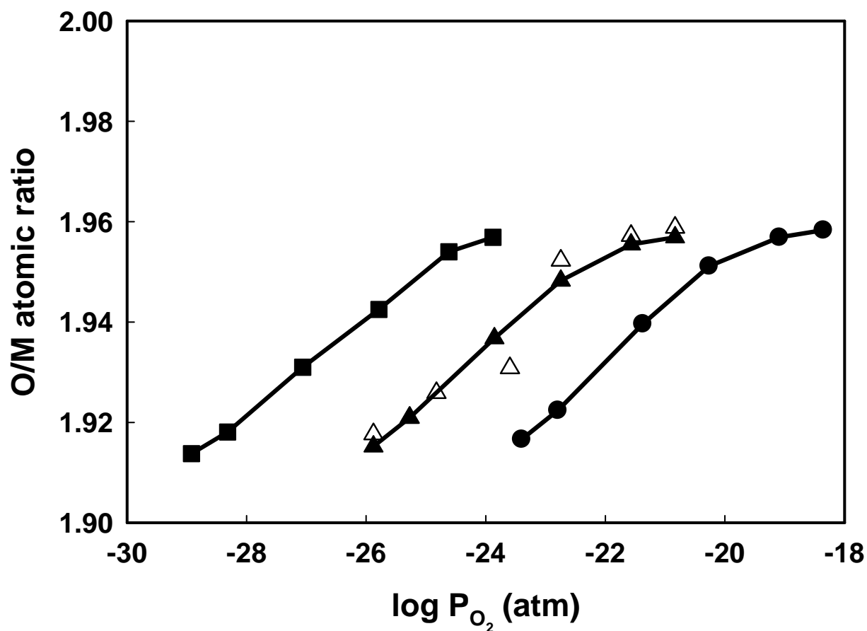
Figure 4d). Oxygen-to-total-metal (Ce+Zr) ratio for 1wt% Pd on Ce_{0.14}Zr_{0.86}O_2 as a function of P(O_2) and temperature (■ 873K, ▲ 973K, ● 1073K). The open symbol ( \Delta ) was obtained on the Ce_{0.14}Zr_{0.86}O_2 with no Pd at 973 K.
