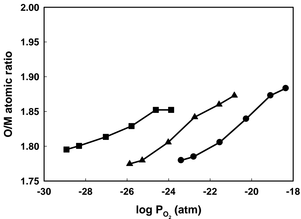
Figure 4b). Oxygen-to-total-metal (Ce+Zr) ratio for \text{Ce}_{0.5}\text{Zr}_{0.5}\text{O}_2 as a function of P(\text{O}_2) and temperature (■ 873K, ▲ 973K, ● 1073K).
