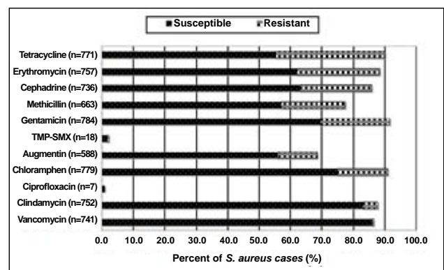
Fig. 2. Antibiotic susceptibility profiles for S. aureus , 2000 - 2007. Antimicrobial susceptibility data were not available at all times. This is why no row reaches 100%.
