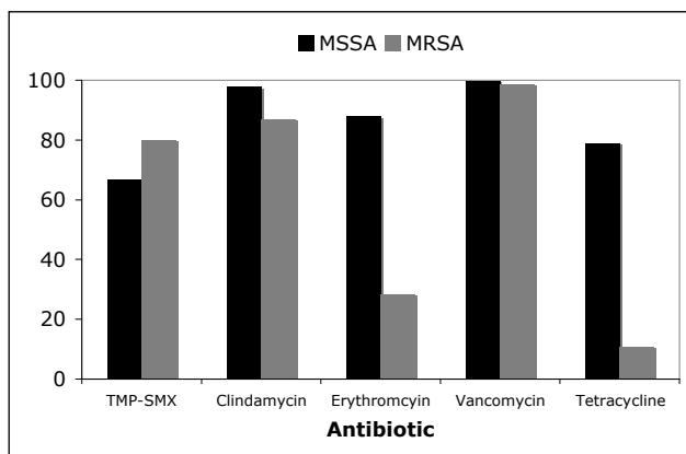
Fig. 3. Comparative susceptibility profiles of MRSA and MSSA.
