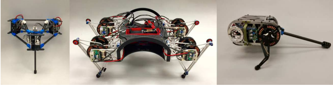
Fig. 1. The DD robots discussed in this paper: Delta Hopper (left), Minitaur (center), and Jerboa (right).
