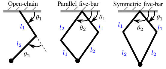
Fig. 4. Leg designs considered in Section II-B.
