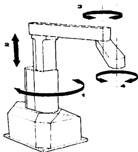
Figure 6: The GMF Model A-500
