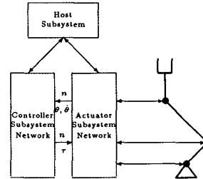
Figure 5: Control System Structure
