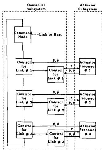
Figure 7: A Controller Hardware Topology.
