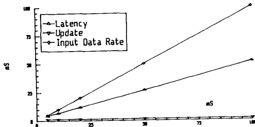
Figure 4: Update and Latency vs Data Input Rate.
