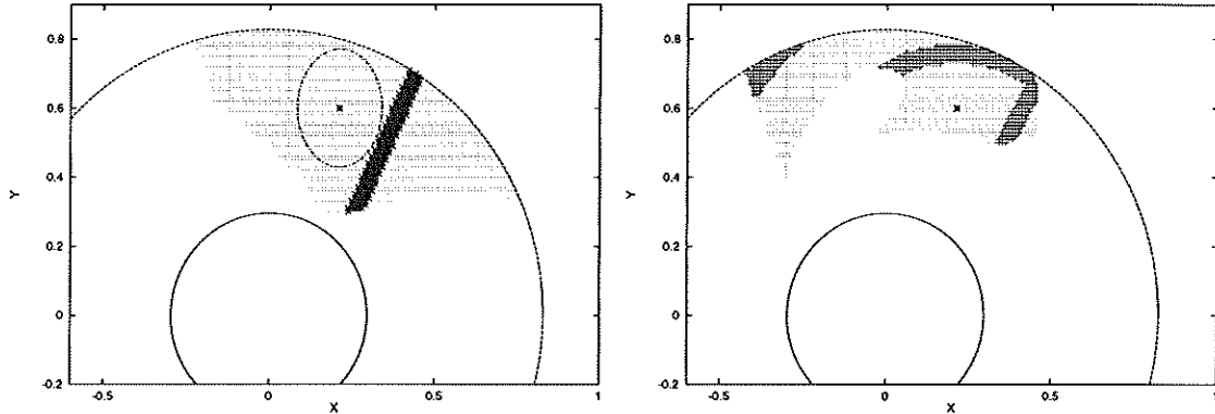
Figure 13: Safe domain for \Phi_{J_0} with the Beam inserted. Light gray areas represent successful initial states, darker areas show states that eventually hit the Beam. (a) Zero initial velocity. The appropriate slice of \mathcal{D}_0 has been added for comparison. (b) \dot{x}_i = 1.5 \frac{m}{s} , showing preimages of the Beam.
