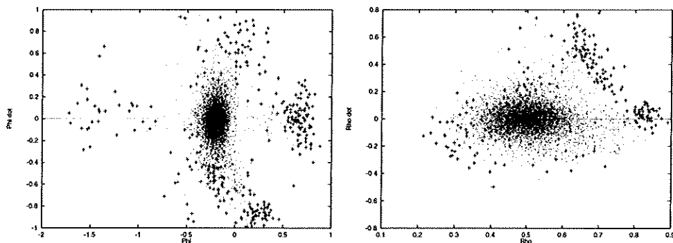
Figure 9: Numerically derived estimate for the horizontally safe juggling domain. The symbol(s) “+” (“.”) denote(s) the points which failed (succeeded) in remaining within the robot’s annular and visible workspace under the action of the numerical simulation of \Phi_J .
