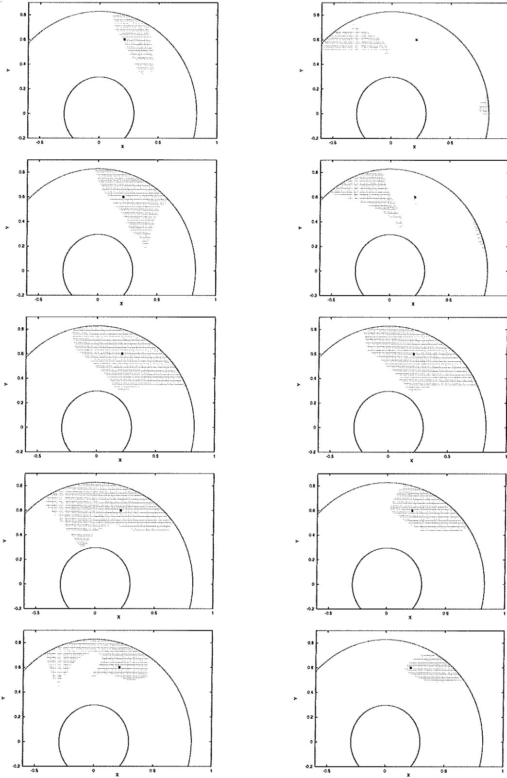
Figure 11: Velocity “spines” – projections onto the zero-velocity plane of slices of \mathcal{H} at regularly spaced velocities – of the invariant attracting domain of \Phi_J . Shaded regions denote initial conditions that were successfully contained in the workspace while being brought to the goal via iterates of f_{\Phi_J} . (a) Left Column: Varying initial \hat{x}_i from negative (top) to positive (bottom) with \hat{y}_i = 0 . (b) Right Column: Varying initial \hat{y}_i from negative to positive with \hat{x}_i = 0 .
