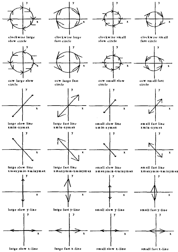
Figure 2: The 24 Gesture Lexicon.
