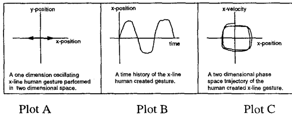
Figure 3: Plots of a Human Create One Dimensional X-Line Oscillating Motion
