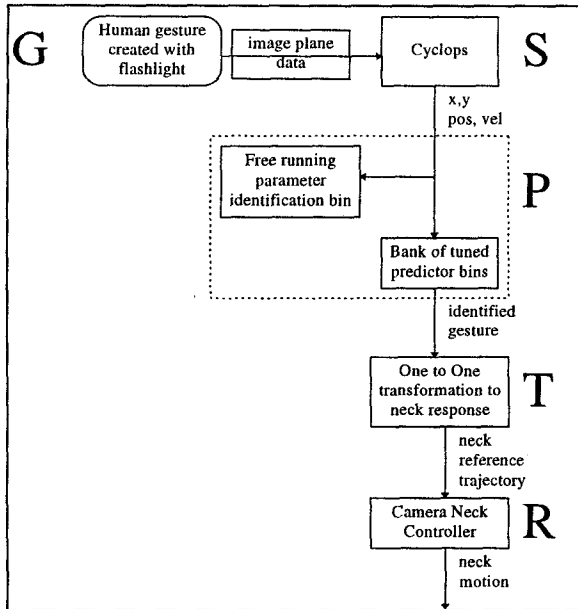
Figure 6: Gesture Recognition System Architecture
