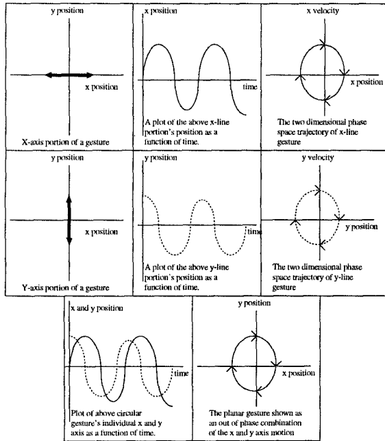
Figure 4: Formation of a Circular Gesture.
