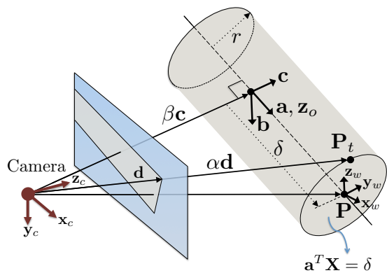
Fig. 2. The geometry of the camera-cylinder system. The coordinate systems of the camera, cylinder object, and world are given by (x_c, y_c, z_c) , (b, c, a) , and (x_w, y_w, z_w) , respectively. The axis of the cylinder \mathbf{a} and the point on the axis closest to the camera, \beta\mathbf{c} , can be estimated directly from the lines representing the boundaries of the cylinder in the image. Further, we assume that the projection \mathbf{d} of a ray passing through the camera and tangent to the cylinder at the \mathbf{a}^T \mathbf{X} = \delta plane can be observed.
