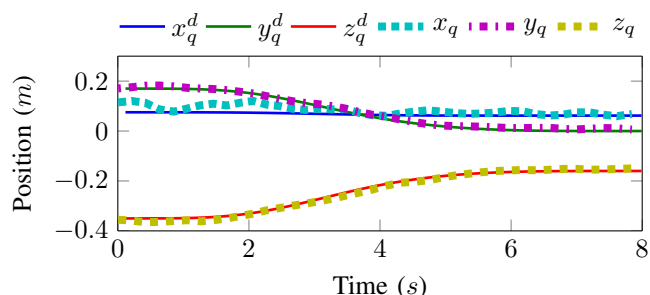
Fig. 10. The desired (computed from \rho_1^d, \rho_2^d , and u^d ) and computed estimate of the quadrotor’s position in the virtual frame \mathcal{V} for a perching maneuver.
